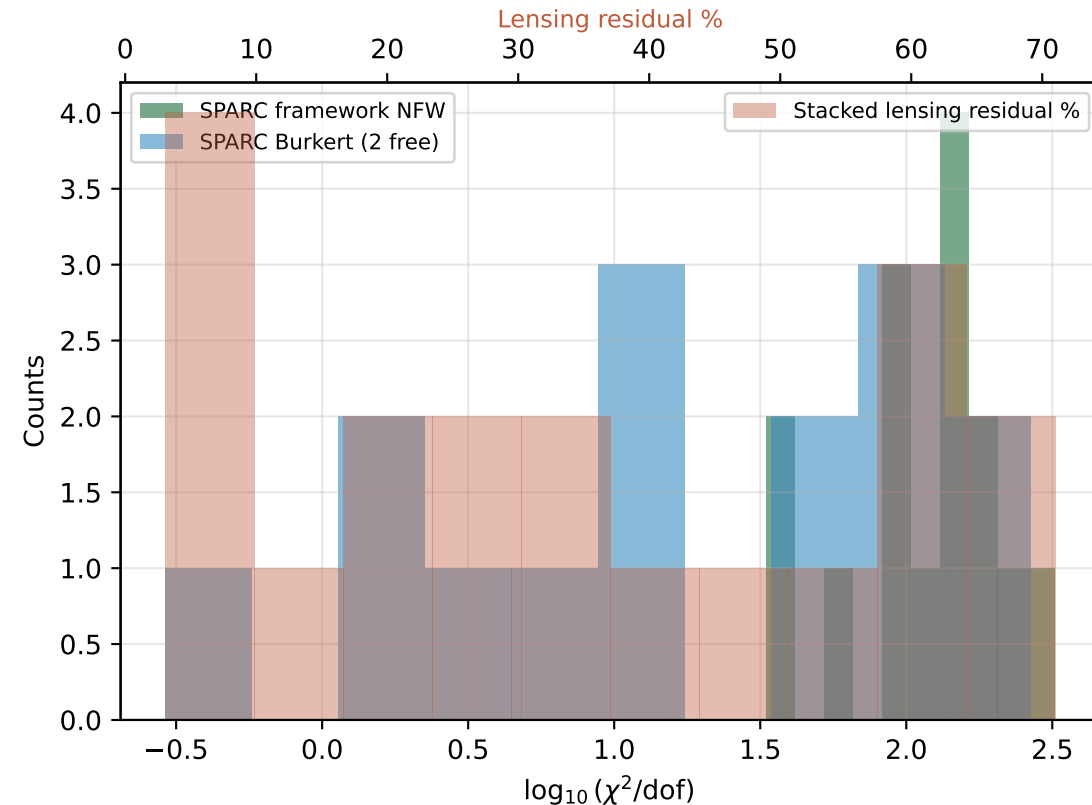
D. Residual distributions: SPARC + lensing
