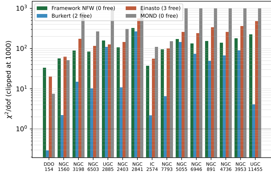
A. SPARC galaxy-by-galaxy fit quality (15 galaxies, dwarf to massive)
