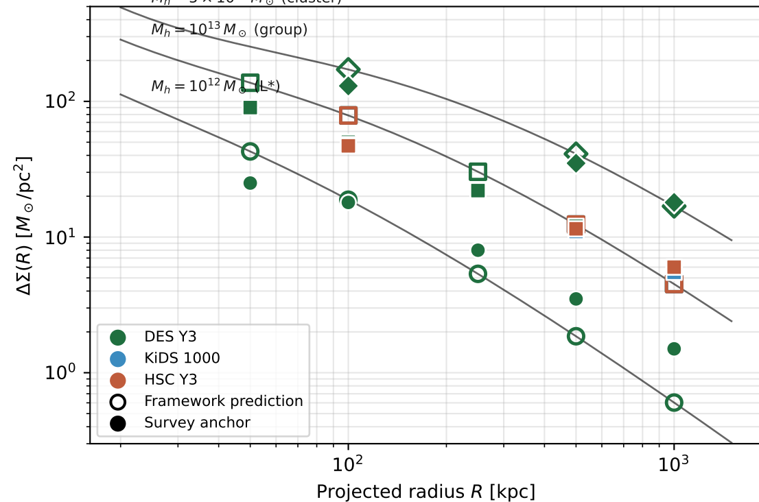
C. Stacked weak-lensing \Delta\Sigma(R) : framework vs DES/KIDS/HSC
