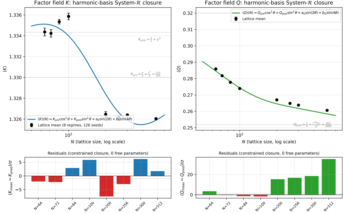
Figure 10: Eight-coefficient System- \mathcal{R} closure of the lattice fixpoints \langle K \rangle(N) and \langle Q \rangle(N) in the natural chirality-flip harmonic basis \{\cos^2\theta, \sin^2\theta, \sin(2\theta), \sin(4\theta)\} . Top: lattice means \pm per-seed standard error on the canonical-physics ladder N \in [64, 512] (8 regimes, 126 seeds), with the parameter-free closure curve Eq. (20) (all four endpoint and four flip-asymmetry coefficients fixed at the System- \mathcal{R} rational targets of Eq. (21)). Endpoint values \{K_{\text{pre}}, K_{\text{post}}, Q_{\text{pre}}, Q_{\text{post}}\} are indicated as horizontal dotted lines. Bottom: per-regime residuals in seed-error units; positive (negative) residuals are coloured blue/green (red). Each of the eight coefficients matches its System- \mathcal{R} rational target at |\Delta|/\sigma \leq 0.40 , parameter-free in (\gamma, N_{\text{gen}}, d) . Generated by src/make_fig_KQ_harmonic_closure.py from the bundled NPZ data and the eight rational targets.
