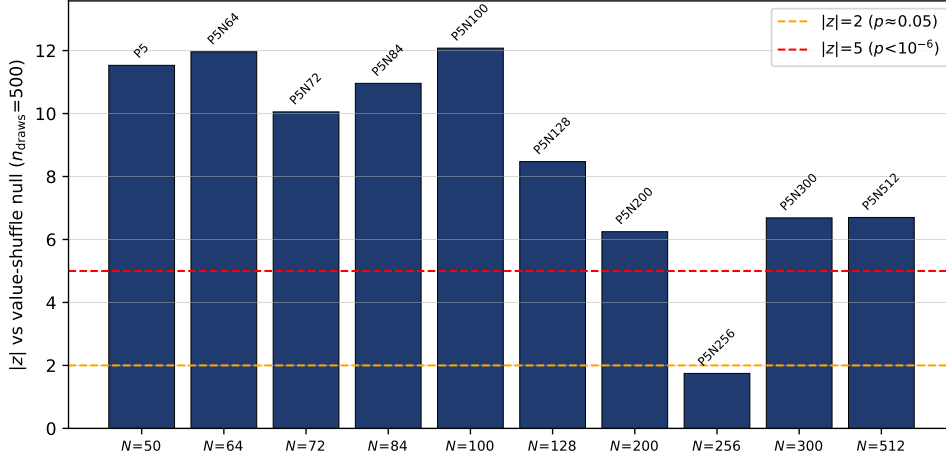
Value-shuffle null on \rho(|R_{00}|, d_{\text{nearest}}) : clean centred-at-zero null, |R_{00}| -halo significant on small-to-mid N , weakens at very large N as R_{00} acquires sign flips
