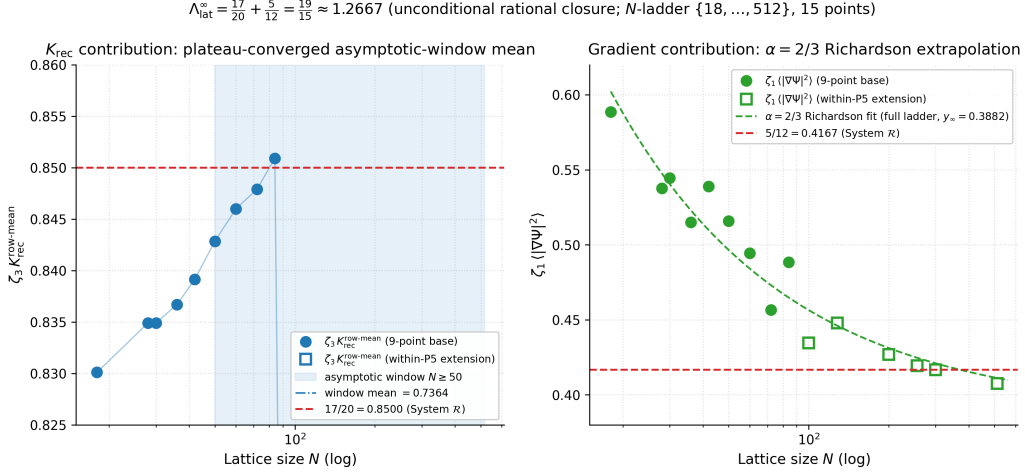
Figure 2: Per-component decomposition of the lattice cosmological-input \Lambda_{\text{lat}}^\infty on the extended ladder N \in \{18, 28, 30, 36, 42, 50, 60, 72, 84, 100, 128, 200, 256, 300, 512\} (9-point base + within-P5 extension, filled vs. open markers; parent paper Figure 7, reproduced here as the source-side cross-witness for the DM/DE mixture decomposition discussed in Section 3).
