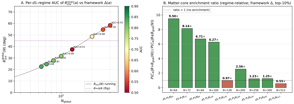
Figure 17: Local RG-window audit of the chirality-flip per-node identity. Panel A: per-regime AUC of \theta_{\text{chir}}(a) from Eq. (58) as predictor of the per-node matter-core indicator (top-decile residual-tail \Delta(a) ), overlaid on the global \theta_{\text{chir}}(N) running curve. Panel B: matter-core enrichment ratio P(C_N|\theta > \pi/4)/P(C_N|\theta \leq \pi/4) across the canonical d1 \mathcal{P}_5 N-ordered ladder at N = 64, 72, 84, 100, 128, 200, 256, 300, 512 (alt-anchor \mathcal{P}_6/\mathcal{P}_8 regimes excluded); values above 1 indicate matter-side nodes are more likely to lie in C_N .
