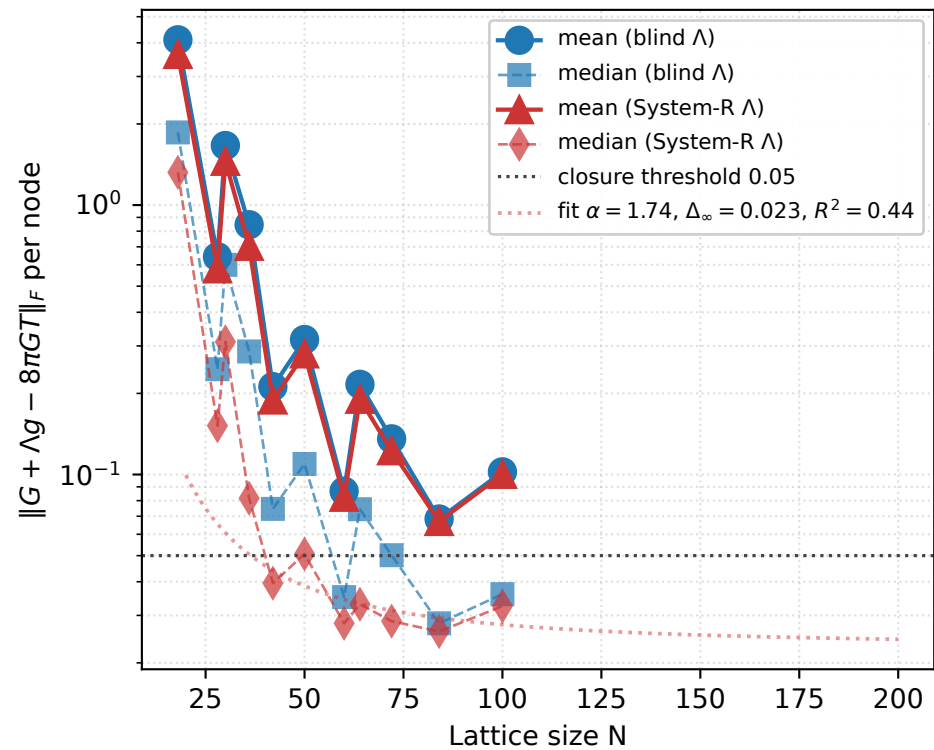
Per-node 4x4 Galerkin Frobenius residual (Hessian-Ricci)
