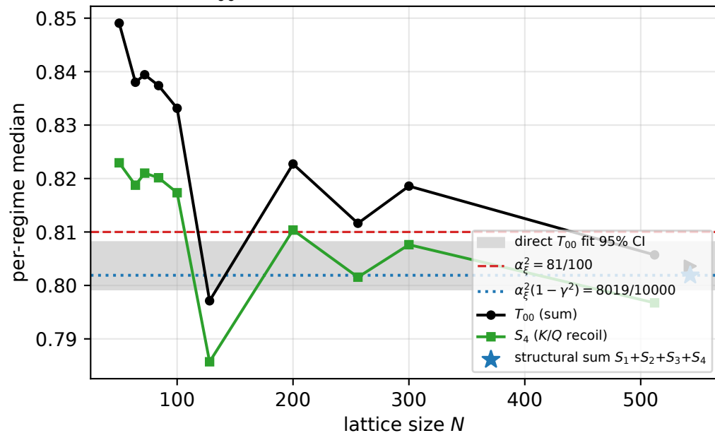
(a) T_{00}^{\Xi} aggregate and dominant summand
