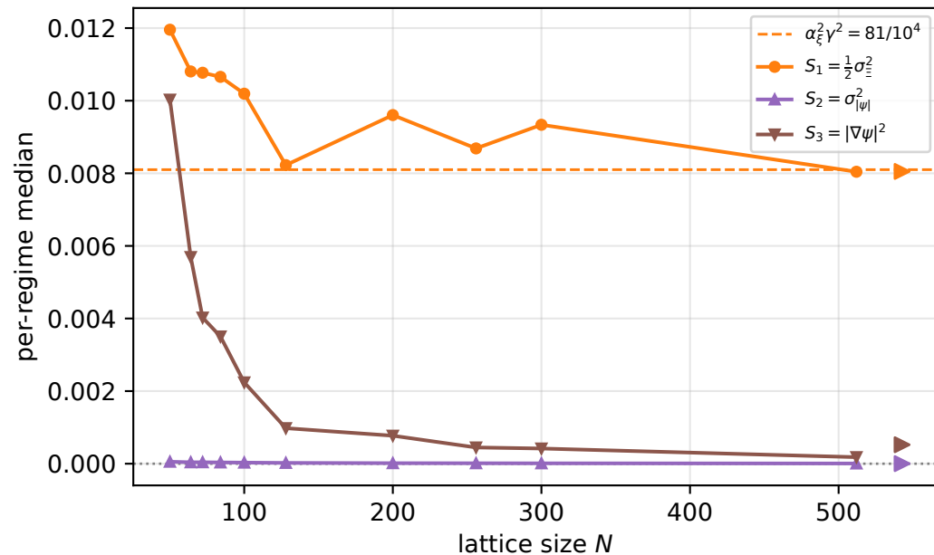
(b) sub-leading summands S_1, S_2, S_3
