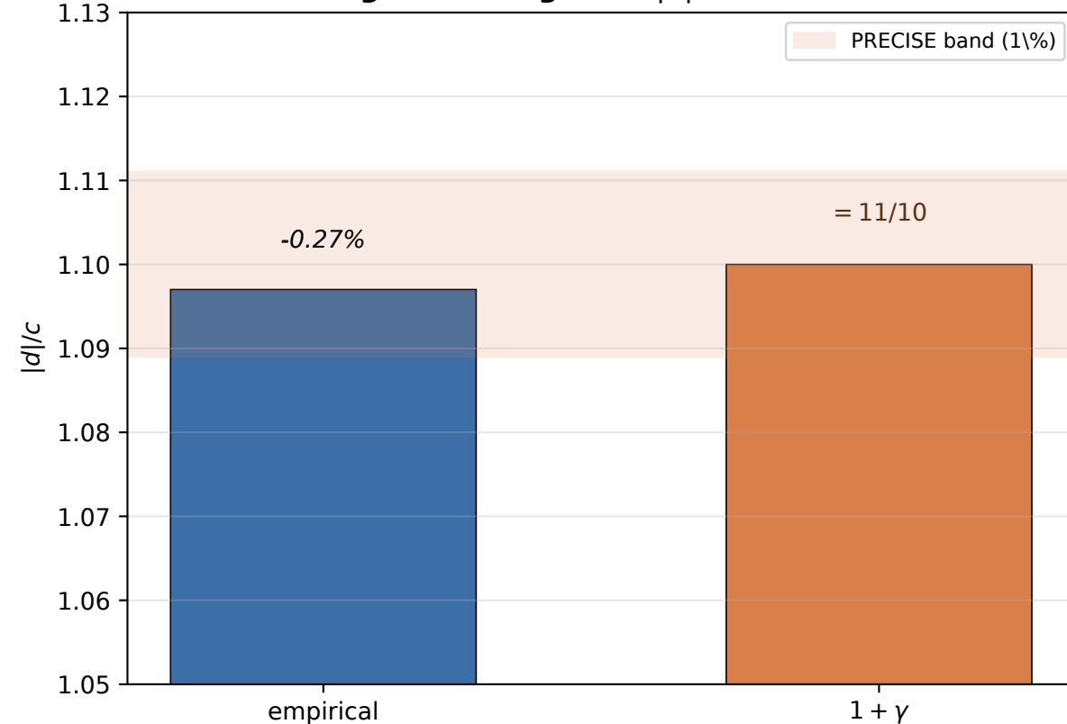
(B) Sub-leading-to-leading ratio |d|/c
