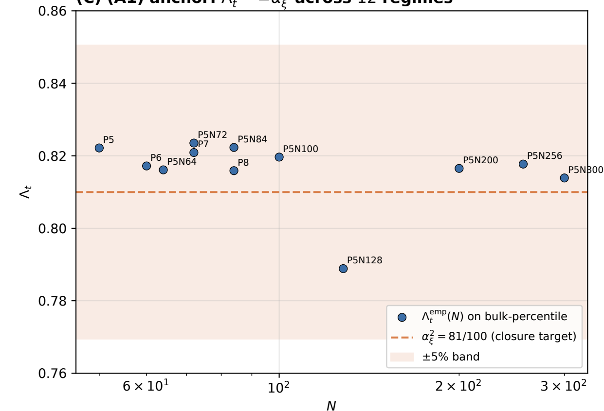
(C) (A1) anchor: \Lambda_t^{\text{emp}} = \alpha_\xi^2 across 12 regimes
