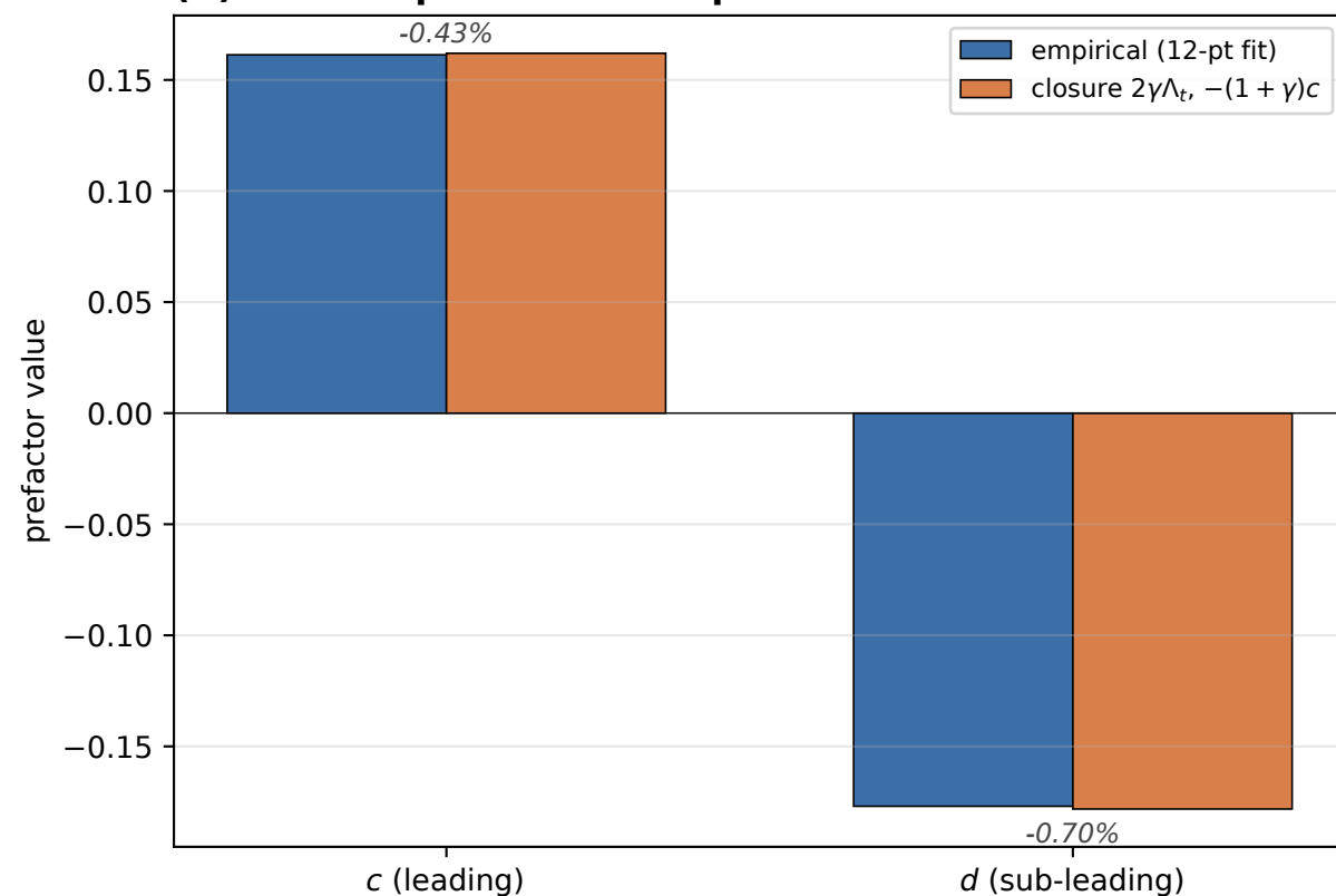
(A) Federer prefactors: empirical vs closure
