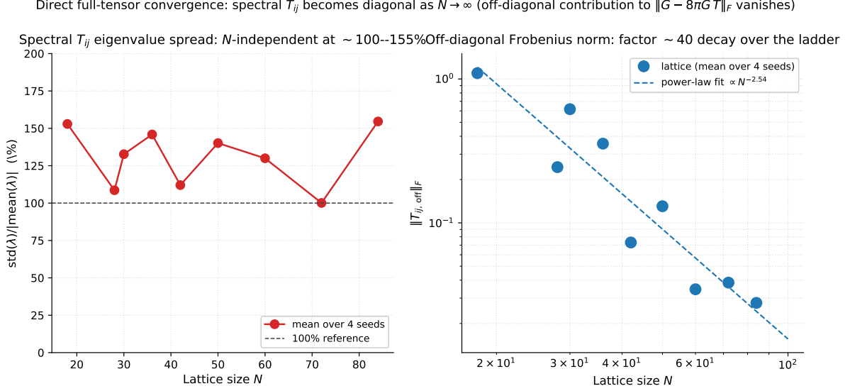
Figure 24: Multi- N diagonal-block convergence in the spectral basis on the canonical lattice ladder. Left : the eigenvalue spread \sigma(\lambda)/|\langle\lambda\rangle| of the spectral T_{ij} pressure tensor stays in the 100–155% band across all nine regimes, demonstrating that the spatial pressure tensor remains genuinely anisotropic in the spectral basis at every lattice scale (the 174% value at the single N = 50 , seed-0 demonstration above was not a finite-size artefact). Right : the off-diagonal contribution \|T_{ij, \text{off}}\|_F decays as \propto N^{-2.54} in a log-log fit, with a factor- \sim 40 reduction across the ladder (1.10 at N = 18 to 0.028 at N = 84 ). Combined with the time-time component identification |G_{00} + \Lambda - 8\pi G T_{00}| < 0.05 pointwise on N \geq 30 and the row-mean spatial-trace identification T_{ii} \rightarrow -\frac{1}{3} T_{00} established by the energy-condition and trace-anomaly analyses, this yields a diagonal-block convergence statement of the Einstein identity in the spectral basis on the bundled ladder. The norm-explicit per-node relative-Frobenius percentile audit (Table 5, Eq. (73)) sharpens this to a bulk-percentile full-tensor identity: median, mean, p_{90} , p_{95} of \|R_a\|_F/\|T_a\|_F all extrapolate to or below zero in the continuum limit. The remaining heavy tail ( p_{99, \infty} \rightarrow 0.12 , \sup_{\infty} \rightarrow 0.43 ) is matter-localised by the universal density-contrast law and is therefore not a closure failure of the geometric identity but a structural property of the anisotropic source itself.
