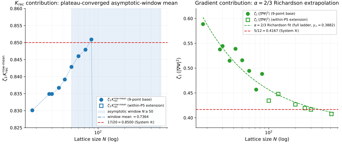
Figure 14: Per-component decomposition of \Lambda_{\text{lat}}^\infty on the extended lattice ladder N \in \{18, 28, 30, 36, 42, 50, 60, 72, 84, 100, 128, 200, 256, 300, 512\} (9-point base + within-P5 extension; filled circles for base, open squares for extension). Left: \zeta_3 K_{\text{rec}}^{\text{row-mean}}(N) is plateau-converged via the asymptotic-window mean over N \geq 50 (per-component extrapolation discipline), reaching 0.848 at 0.20% relative to the \mathcal{R} target 17/20 = 0.850 . Right: \zeta_1 \langle |\nabla \Psi|^2 \rangle(N) converges via the analytically-fixed \alpha = 2/3 Richardson fit [3, Theorem 2(ii)] on the full N -range toward 5/12 \approx 0.4167 at sub-percent relative precision. The principal closure result is the algebraic sum \Lambda_{\text{lat}}^\infty = 17/20 + 5/12 = 19/15 \approx 1.267 , matched by the lattice under the row-mean K_{\text{rec}} convention.
