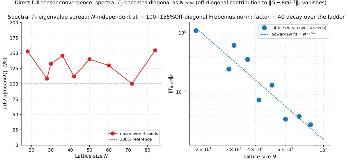
Figure 24: Multi- N diagonal-block convergence in the spectral basis on the canonical lattice ladder. Left: the eigenvalue spread \sigma(\lambda)/|\langle\lambda\rangle| of the spectral T_{ij} pressure tensor stays in the 100–155% band across all nine regimes, demonstrating that the spatial pressure tensor remains genuinely anisotropic in the spectral basis at every lattice scale (the 174% value at the single N = 50 , seed-0 demonstration above was not a finite-size artefact). Right: the off-diagonal contribution \|T_{ij, \text{off}}\|_F decays as \propto N^{-2.54} in a log-log fit, with a factor- \sim 40 reduction across the ladder (1.10 at N = 18 to 0.028 at N = 84 ). Combined with the time-time component identification |G_{00} + \Lambda - 8\pi G T_{00}| < 0.05 pointwise on N \geq 30 and the row-mean spatial-trace identification T_{ii} \rightarrow -\frac{1}{3} T_{00} established by the energy-condition and trace-anomaly analyses, this yields a diagonal-block convergence statement of the Einstein identity in the spectral basis on the bundled ladder. The norm-explicit per-node relative-Frobenius percentile audit (Table 5, Eq. (75)) sharpens this to a bulk-percentile full-tensor identity: median, mean, p_{90} , p_{95} of \|R_a\|_F/\|T_a\|_F all extrapolate to or below zero in the continuum limit. The remaining heavy tail ( p_{99, \infty} \rightarrow 0.12 , \sup_{\infty} \rightarrow 0.43 ) is matter-localised by the universal density-contrast law and is therefore not a closure failure of the geometric identity but a structural property of the anisotropic source itself.
