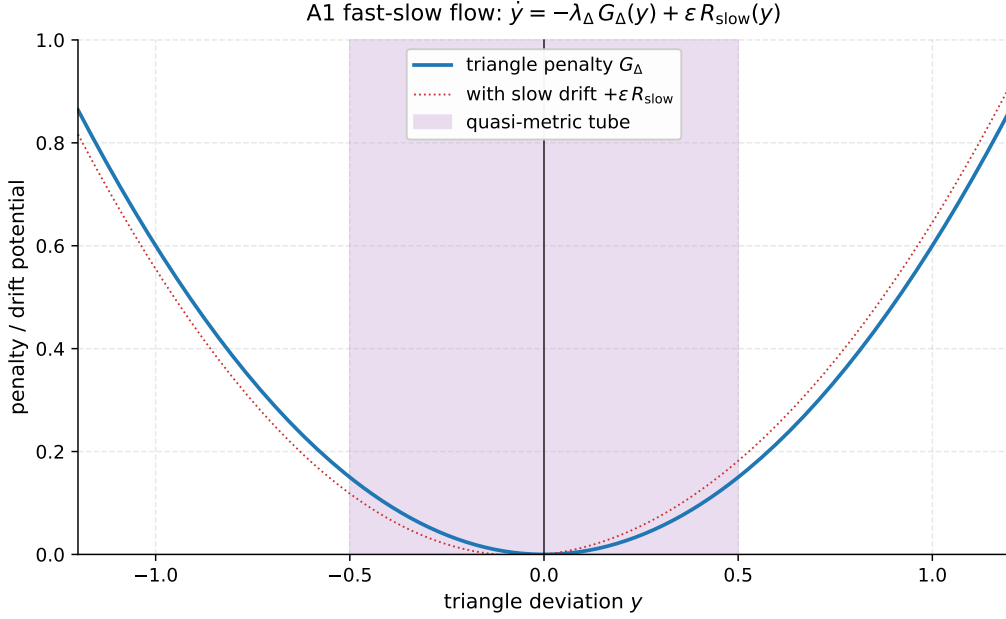
Figure 7: Fast-slow gradient flow. The blue curve is the triangle penalty G_\Delta near the sub-multiplicative regime; the dotted red curve is the same with the slow drift \epsilon R_{slow} added. The shaded purple band is the quasi-metric tube into which the flow funnels.
