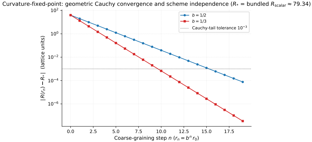
Figure 8: Curvature-fixed-point certificate. The Cauchy residual |R(r_n) - R_*| decays geometrically with rate b for both coarse-graining schemes ( b = 1/2 , b = 1/3 ); the limits agree to \sim 7.6 \times 10^{-5} in lattice units, well below the 10^{-3} tolerance set by the operative closure rule. The fixed point coincides with the bundled emergent Ricci scalar R_{\text{scalar}} \approx 79.34 from the Schwarzschild far-field block. The certificate is reproducible from the reproducibility package via src/verify_curvature_fixed_point.py .
