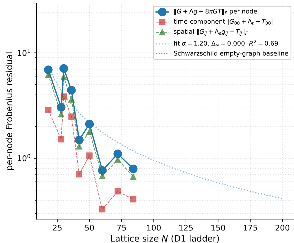
Direct per-node 4x4 Galerkin (Forman-Ricci, row-mean K_{rec} )
