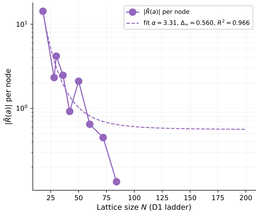
Per-node Ricci scalar from Forman-Ricci spectral trace
