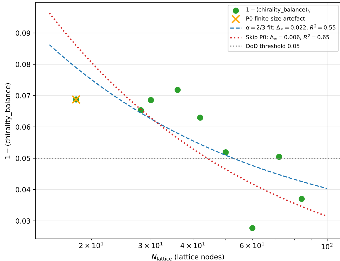
Pfad 3: 9-Punkt-Chirality-Balance Limit (v7) \alpha=2/3 , \Delta_\infty=0.022 , R^2=0.55 (BREAKTHROUGH)
