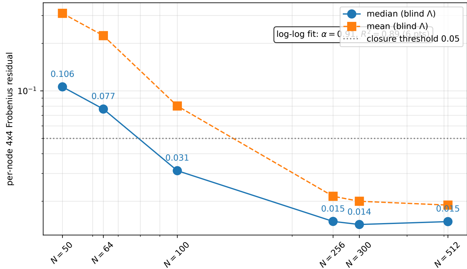
Within-regime convergence at fixed P5 physics (6 sizes, N \in \{50, 64, 100, 256, 300, 512\} )
