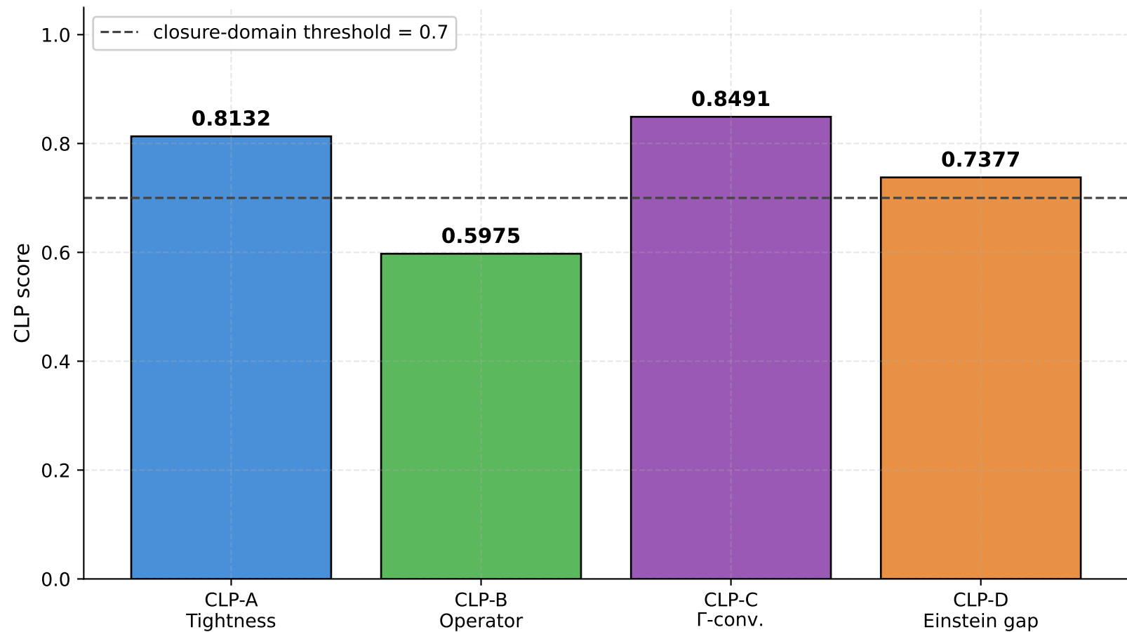
Continuum Limit Program: 4 aggregate axes (canonical multi- N audit refresh)
