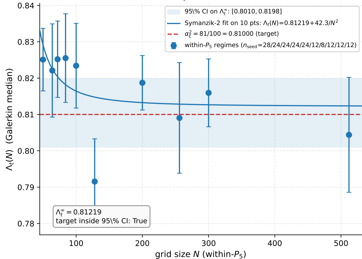
(b) Within- P_5 Symanzik-2 fit of \Lambda_t on 10 points N \in [50, 512] : algebraic target \alpha_\xi^2 inside 95% bootstrap CI
