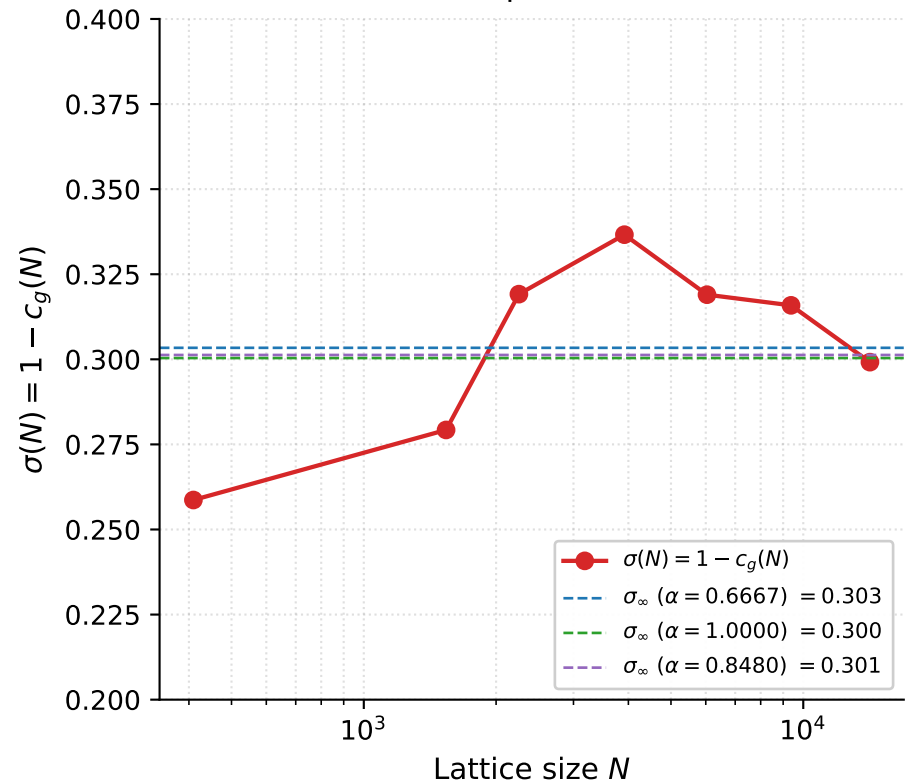
Discrete metric-stress profile, \sigma(N) \in [0.26, 0.34]
