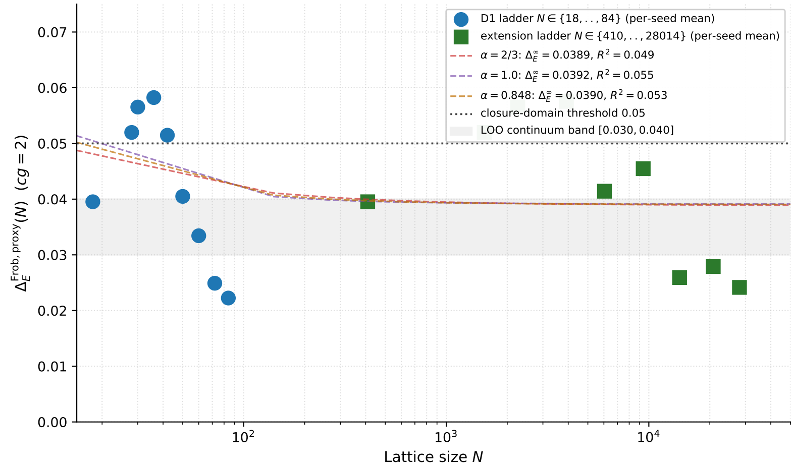
Eighteen-point Frobenius-decomposed proxy: \emph{bounded floor} in [0.022, 0.058] across factor- \sim 1556 in N
