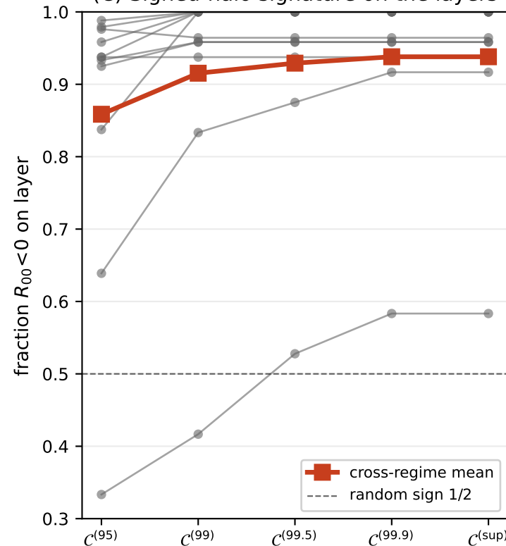
(C) Signed-halo signature on the layers
