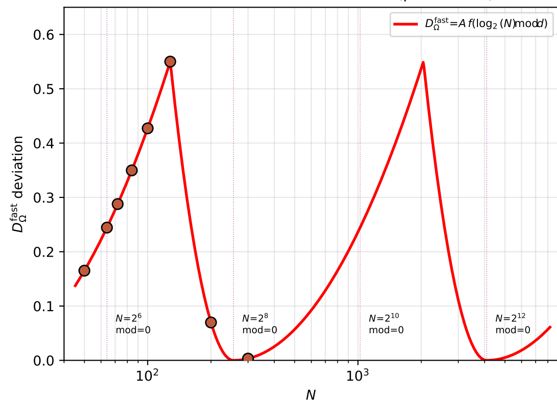
C. FAST lattice-harmonic oscillation (period d=4 )
