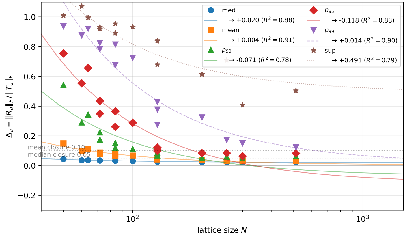
Bulk-percentile full-tensor closure: per-node relative-Frobenius residual canonical \mathcal{P}_5/\mathcal{P}_5N ladder N \in [50, 512] (10 regimes, 180 seeds) + alt-anchor cross-check (5 regimes, 88 seeds)
