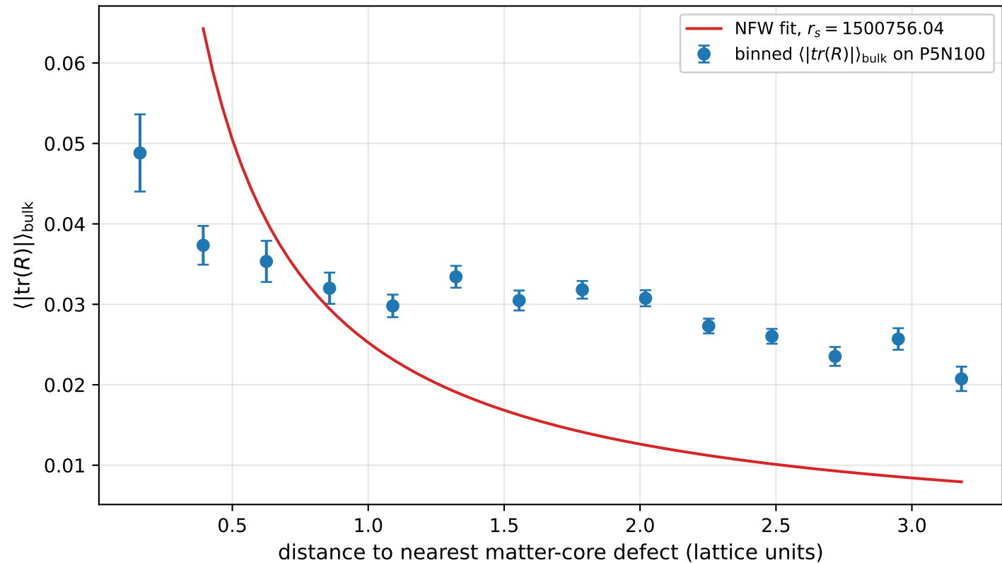
Radial profile of the bulk signed-trace amplitude around defects (P5N100)
