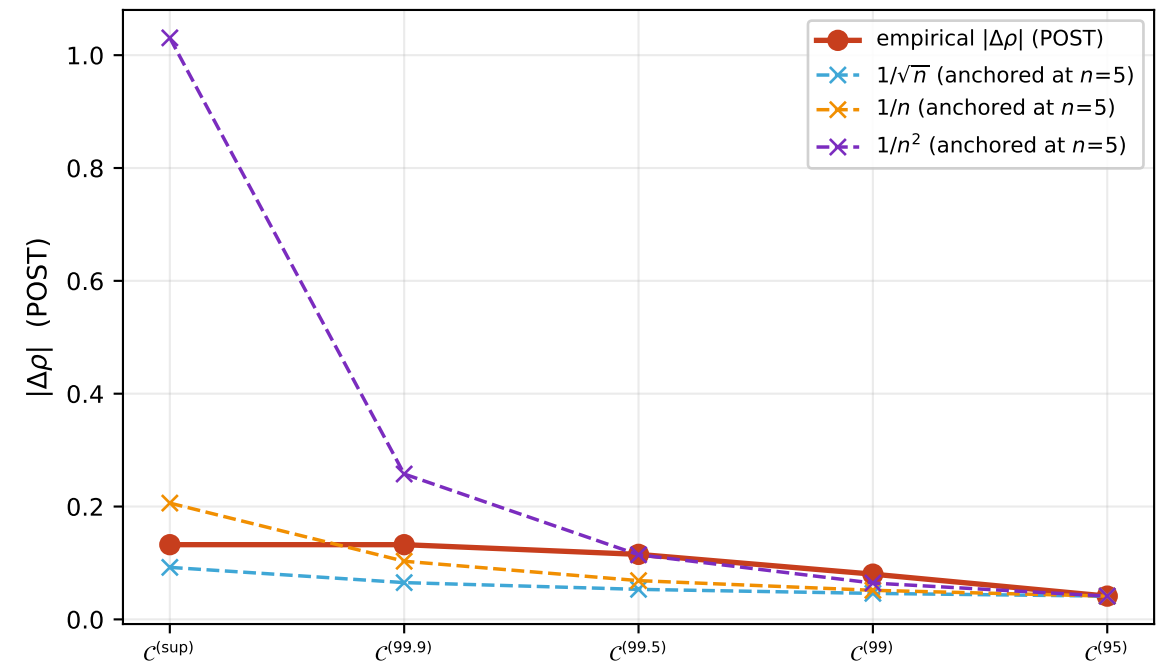
(B) |\Delta\rho| vs candidate n -scalings: 1/\sqrt{n} best fit
