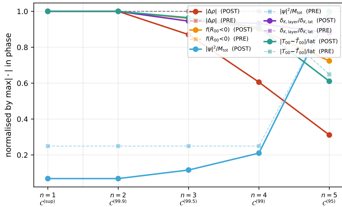
(A) Five diagnostics across shell rank n , PRE (dashed) vs POST (solid)
