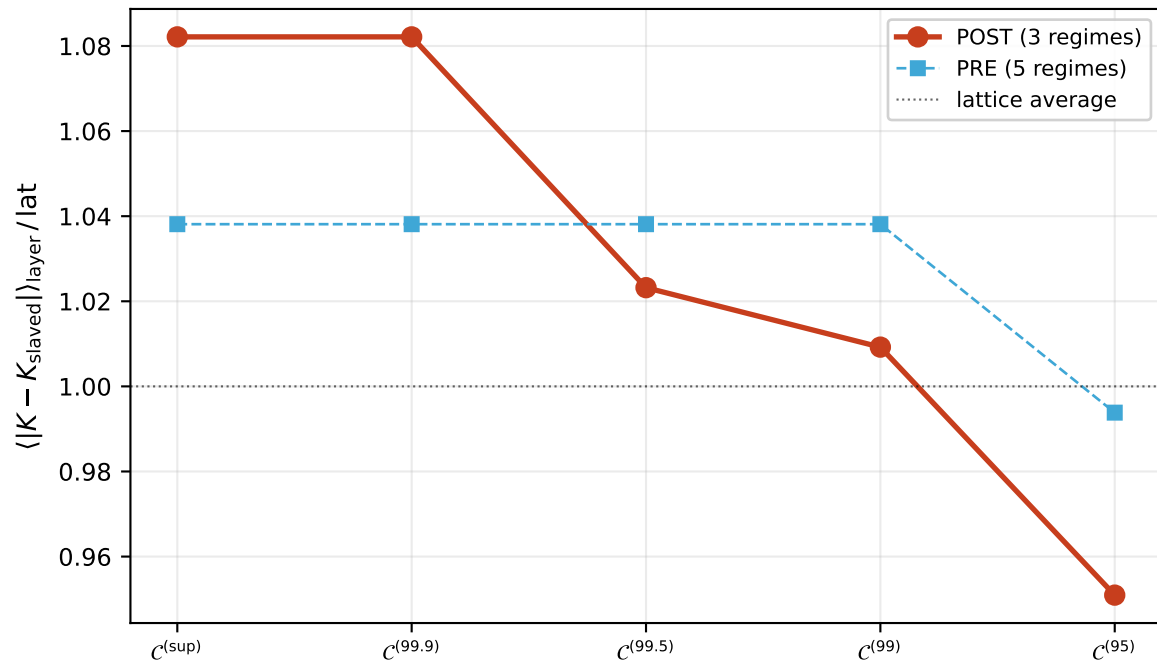
(C) Slaving- K residual ratio per layer (unslavedness)
