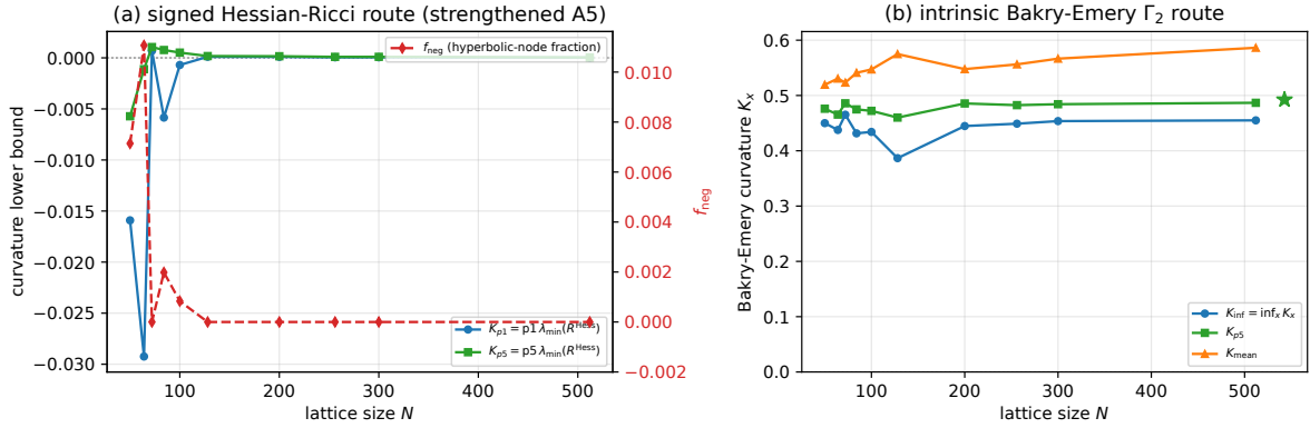
Figure 16: Empirical witnesses of the curvature-dimension lower bound CD(K_{\text{CD}}, N) on the canonical-physics ladder N \in [50, 512] , the two routes named in the proof of Theorem 13. (a) Strengthened-(A5) route ( src/verify_signed_ricci_lower_bound.py ): the robust percentile lower bounds K_{p1}, K_{p5} of the signed Hessian-discrepancy Ricci minimum eigenvalue extrapolate to a finite limit with a non-negative point estimate (bootstrap CI straddling zero, hence consistent with CD(0, N) ), and the hyperbolic-node fraction f_{\text{neg}} (red, right axis) vanishes for N \geq 128 . (b) Measure-contraction route ( src/verify_carrier_bakry_emory_cd.py ): the intrinsic Bakry–Émery \Gamma_2 curvature percentiles K_{\text{inf}}, K_{p5}, K_{\text{mean}} of the carrier random-walk Dirichlet form are uniformly positive across the ladder; the robust K_{p5} asymptote (green star) is bounded away from zero. Both routes independently support a uniform CD(K_{\text{CD}}, N) bound with K_{\text{CD}} \geq 0 .
