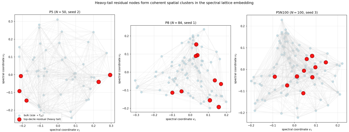
Figure 27: Heavy-tail residual nodes (red, top-decile) form coherent spatial clusters in the two-dimensional spectral embedding ( v_1, v_2 ) of the relational graph at three representative regimes. Bulk nodes (light blue) are sized by local T_{00} . Edges drawn for \Xi_{ab} > \Xi_{\text{thresh}} with width proportional to \Xi_{ab} . The internal mean similarity inside the heavy-tail subset is a factor 2–3 above the global mean, and at N = 100 the ten heavy-tail nodes lie in a single connected component, consistent with a matter-core nucleation reading.
