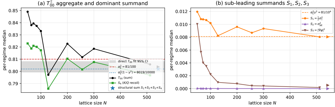
Figure 15: Per-summand continuum decomposition of T_{00}^\Xi on the canonical-physics ladder N \in [50, 512] ( src/verify_t00_summand_decomposition.py ). (a) The noisy aggregate T_{00} and the dominant K/Q -recoil summand S_4 , with the direct-fit bootstrap 95% CI band (grey); the structural sum S_1+S_2+S_3+S_4 = 8019/10000 (blue star) lies inside that band, on \alpha_\xi^2(1-\gamma^2) (blue dotted), while \alpha_\xi^2 = 81/100 (red dashed) sits above it. (b) The three sub-leading summands: the edge- \Xi row-variance term S_1 = \frac{1}{2}\sigma_\Xi^2 lands on \alpha_\xi^2\gamma^2 = 81/10^4 while the amplitude-variance and gradient-energy terms S_2, S_3 vanish. Right-pointing markers are the per-summand Symanzik asymptotes.
