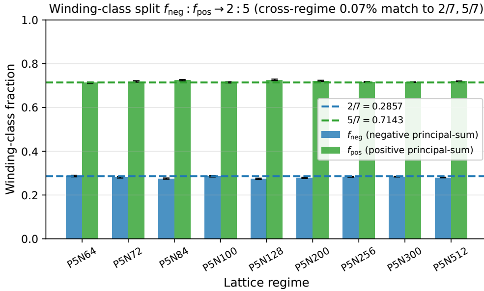
Figure 30: Winding-class fractions f_{\text{neg}} and f_{\text{pos}} = 1 - f_{\text{neg}} per regime on the canonical-physics ladder N \in [64, 512] . Cross-regime Symanzik asymptote f_{\text{neg},\infty} = 0.28552 \pm 0.00081 matches 2/7 = 0.28571 at 0.24\sigma (absolute deviation 2 \times 10^{-4} ). The closed-form derivation (110) via the B_{N_{\text{gen}}} = \mathfrak{so}(2N_{\text{gen}} + 1) short-root fraction is parameter-free.
