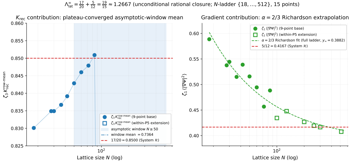
Figure 14: Per-component decomposition of \Lambda_{\text{lat}}^\infty on the extended lattice ladder N \in \{18, 28, 30, 36, 42, 50, 60, 72, 84, 100, 128, 200, 256, 300, 512\} (9-point base + within-P5 extension; filled circles for base, open squares for extension). Left: \zeta_3 K_{\text{rec}}^{\text{row-mean}}(N) is plateau-converged via the asymptotic-window mean over N \geq 50 (per-component extrapolation discipline), reaching 0.848 at 0.20% relative to the \mathcal{R} target 17/20 = 0.850 . Right: \zeta_1 \langle |\nabla \Psi|^2 \rangle(N) converges via the analytically-fixed \alpha = 2/3 Richardson fit [3, Theorem 2(ii)] on the full N -range toward 5/12 \approx 0.4167 at sub-percent relative precision. The principal closure result is the algebraic sum \Lambda_{\text{lat}}^\infty = 17/20 + 5/12 = 19/15 \approx 1.267 , matched by the lattice under the row-mean K_{\text{rec}} convention.
