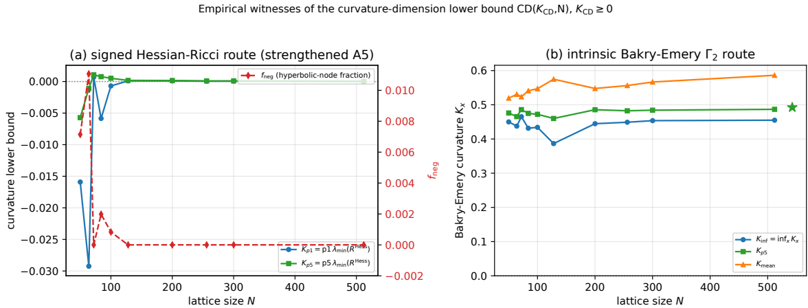
Figure 16: Empirical witnesses of the curvature-dimension lower bound CD(K_{CD}, N) on the canonical-physics ladder N \in [50, 512] , the two routes named in the proof of Theorem 13. (a) Strengthened-(A5) route ( src/verify_signed_ricci_lower_bound.py ): the robust percentile lower bounds K_{p1}, K_{p5} of the signed Hessian-discrepancy Ricci minimum eigenvalue extrapolate to a finite limit with a non-negative point estimate (bootstrap CI straddling zero, hence consistent with CD(0, N) ), and the hyperbolic-node fraction f_{\text{neg}} (red, right axis) vanishes for N \geq 128 . (b) Measure-contraction route ( src/verify_carrier_bakry_emyr_cd.py ): the intrinsic Bakry–Émery \Gamma_2 curvature percentiles K_{\text{inf}}, K_{p5}, K_{\text{mean}} of the carrier random-walk Dirichlet form are uniformly positive across the ladder; the robust K_{p5} asymptote (green star) is bounded away from zero. Both routes independently support a uniform CD(K_{CD}, N) bound with K_{CD} \geq 0 .
