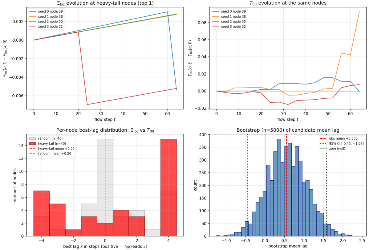
Figure 29: Empirical evidence for the geometric-condensation direction \Xi \rightarrow T_{00} at heavy-tail residual nodes. Top row : per-node time-evolution of \Xi_{\text{loc}}(a, t) (left) and T_{00}(a, t) (right), centred at t = 0 , for the highest-residual node in each of four seeds. Bottom-left : per-node best-lag distribution at candidate (top-decile, red) versus random non-candidate (grey) nodes; the candidate distribution is shifted toward positive lags (mean +0.55, non-candidate mean near 0). Bottom-right : bootstrap distribution of the candidate mean-lag estimate with 95% confidence interval. The five-test detailed audit is at outputs/geometric_condensation_detailed_audit.json .
