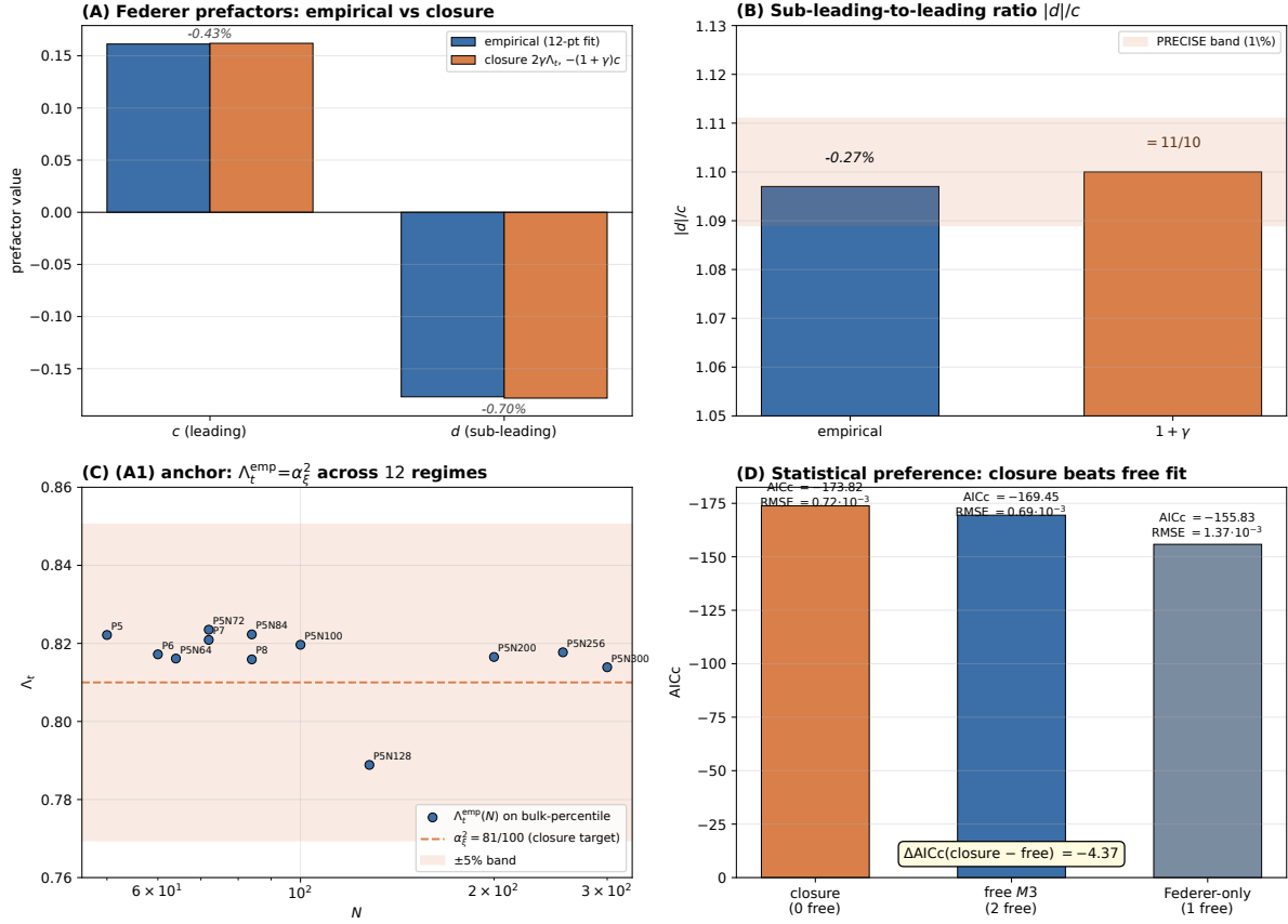
Figure 21: Cross-anchor empirically-derived Federer-prefactor closure on the twelve-point cross-anchor ladder ( P_5, P_5N_{64}, \dots, P_5N_{300} canonical and P_6, P_7, P_8 alt-anchor entries; N \in [50, 300] ). (A) Closed-form identification c = 2\gamma\Lambda_t = 81/500 and d = -(1+\gamma)c = -891/5000 matches the empirical M3 fit at PRECISE tier ( -0.43\% on c , -0.70\% on d ). (B) Sub-leading-to-leading ratio |d|/c : empirical 1.097 vs closure 11/10 ( -0.27\% ). (C) Empirical confirmation of anchor (A1) \Lambda_t = \alpha_\xi^2 : across all twelve regimes the bulk-percentile \Lambda_t^{\text{emp}} stays within \pm 5\% (in fact within \pm 2.5\% ) of \alpha_\xi^2 = 81/100 , demonstrating that the closure is not just an asymptotic landing but a per-regime structural relation. (D) AICc model comparison: the parameter-free closure c = 2\gamma\Lambda_t , d = -(1+\gamma)c beats the unconstrained two-parameter fit at \Delta\text{AICc} = -4.37 , with effectively identical RMSE. The Federer-only single-parameter model is dominated. The alternative shear factorisation c = \alpha_\xi \|T_{\text{off}}\| (not shown; would extend the AICc panel by another +86) is empirically falsified. Reproducer: src/make_fig_federer_prefactor_closure.py ; data bundles outputs/federer_extended_ladder_results.json , outputs/federer_physical_factorization_results.json .
