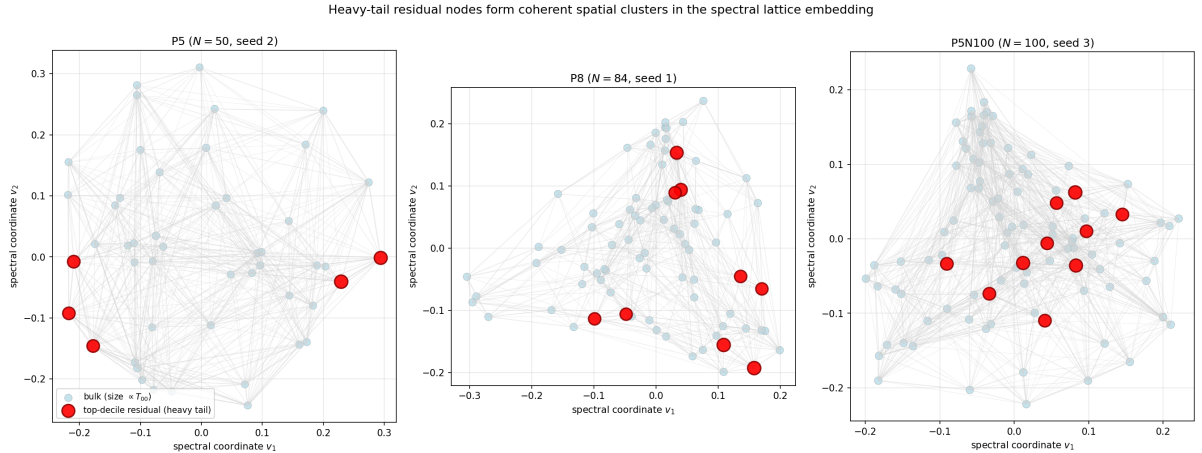
Figure 25: Heavy-tail residual nodes (red, top-decile) form coherent spatial clusters in the two-dimensional spectral embedding (v_1, v_2) of the relational graph at three representative regimes. Bulk nodes (light blue) are sized by local T_{00} . Edges drawn for \Xi_{ab} > \Xi_{\text{thresh}} with width proportional to \Xi_{ab} . The internal mean similarity inside the heavy-tail subset is a factor 2–3 above the global mean, and at N = 100 the ten heavy-tail nodes lie in a single connected component, consistent with a matter-core nucleation reading.
