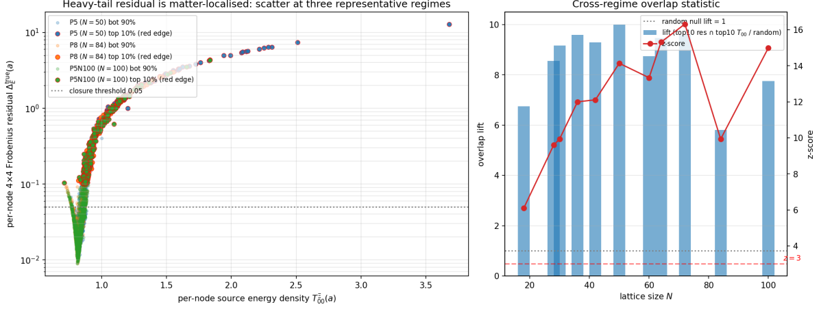
Figure 21: Heavy-tail per-node Frobenius residual is matter-localised. Left : per-node scatter of the residual against the source energy density T_{00}^\Xi(a) at three representative regimes. The top-decile-residual nodes (red-edged points) cluster at the high- T_{00} end of the scatter rather than spreading uniformly. Right : cross-regime overlap statistic for the top-decile-residual / top-decile- T_{00} mask intersection: the lift is 8.6 on average across the 15 audited regimes (10 canonical + 5 alt-anchor) (mean z -score +12.2), demonstrating that the heavy tail is concentrated where the source-tensor magnitude is largest. The analogous test against the topological vortex winding mask gives lift 0.83 ( z = -0.3 , statistically independent), showing that the heavy tail is a continuum-source-magnitude effect, not a topological-defect effect.
