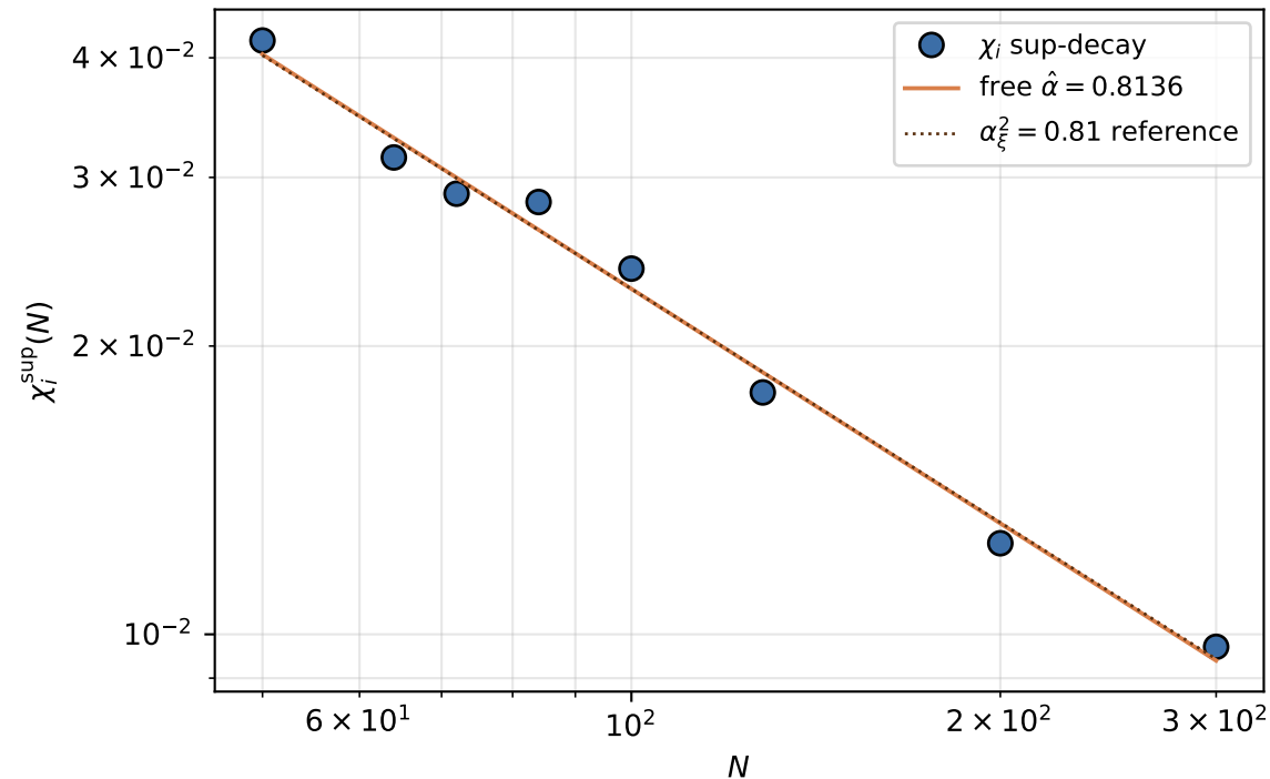
Per-direction chirality sup-decay log-log
