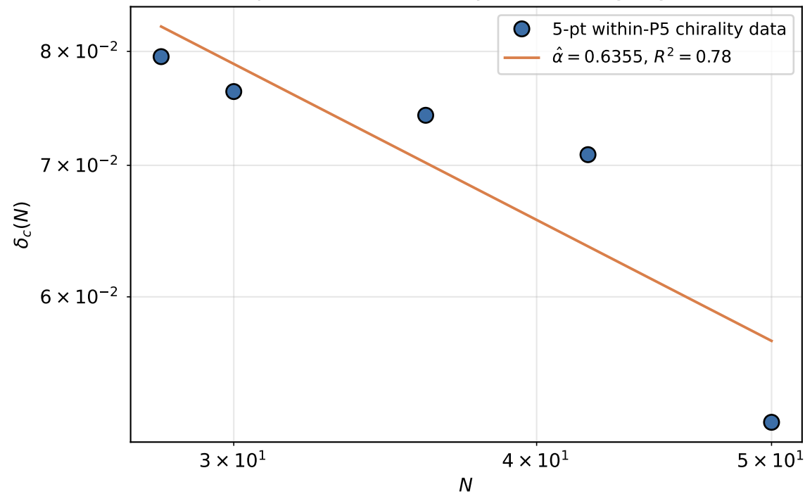
5-pt within-P5 chirality residual log-log fit
