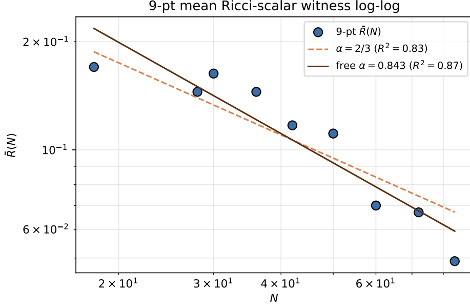
Figure 3: Nine-point mean Ricci-scalar witness log-log fit: fixed- \alpha = 2/3 gives R^2 = 0.83 ; free- \alpha = 0.843 improves to R^2 = 0.87 .
