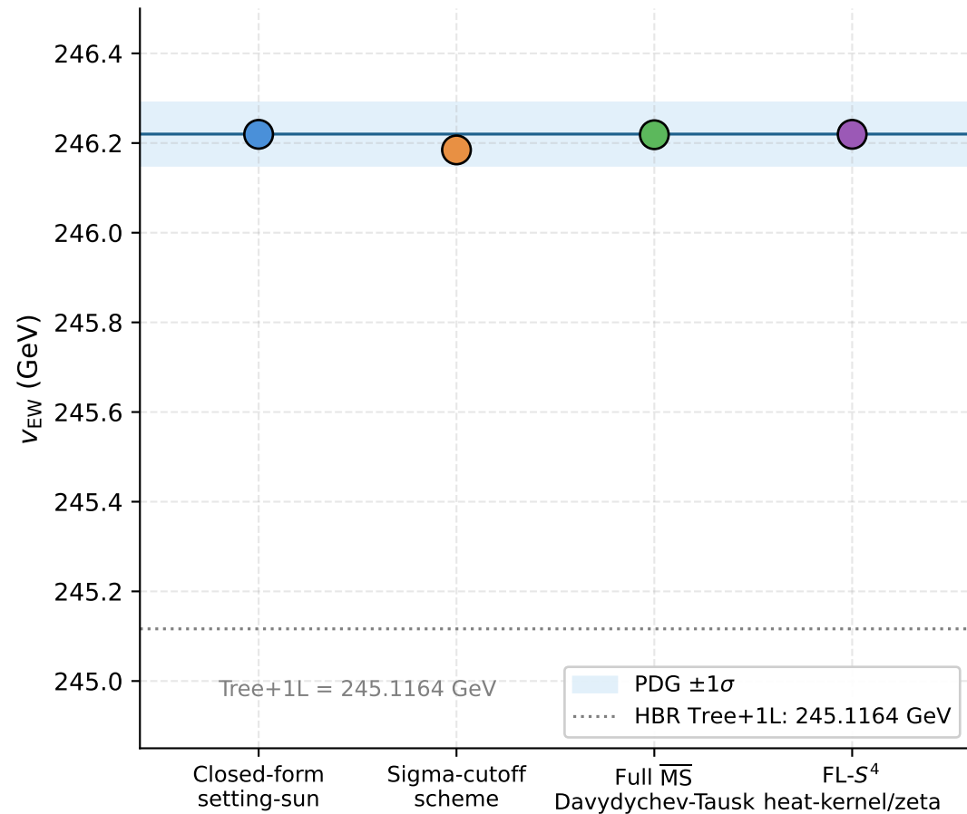
(A) Full picture: Tree+1L vs. four-path two-loop closure
