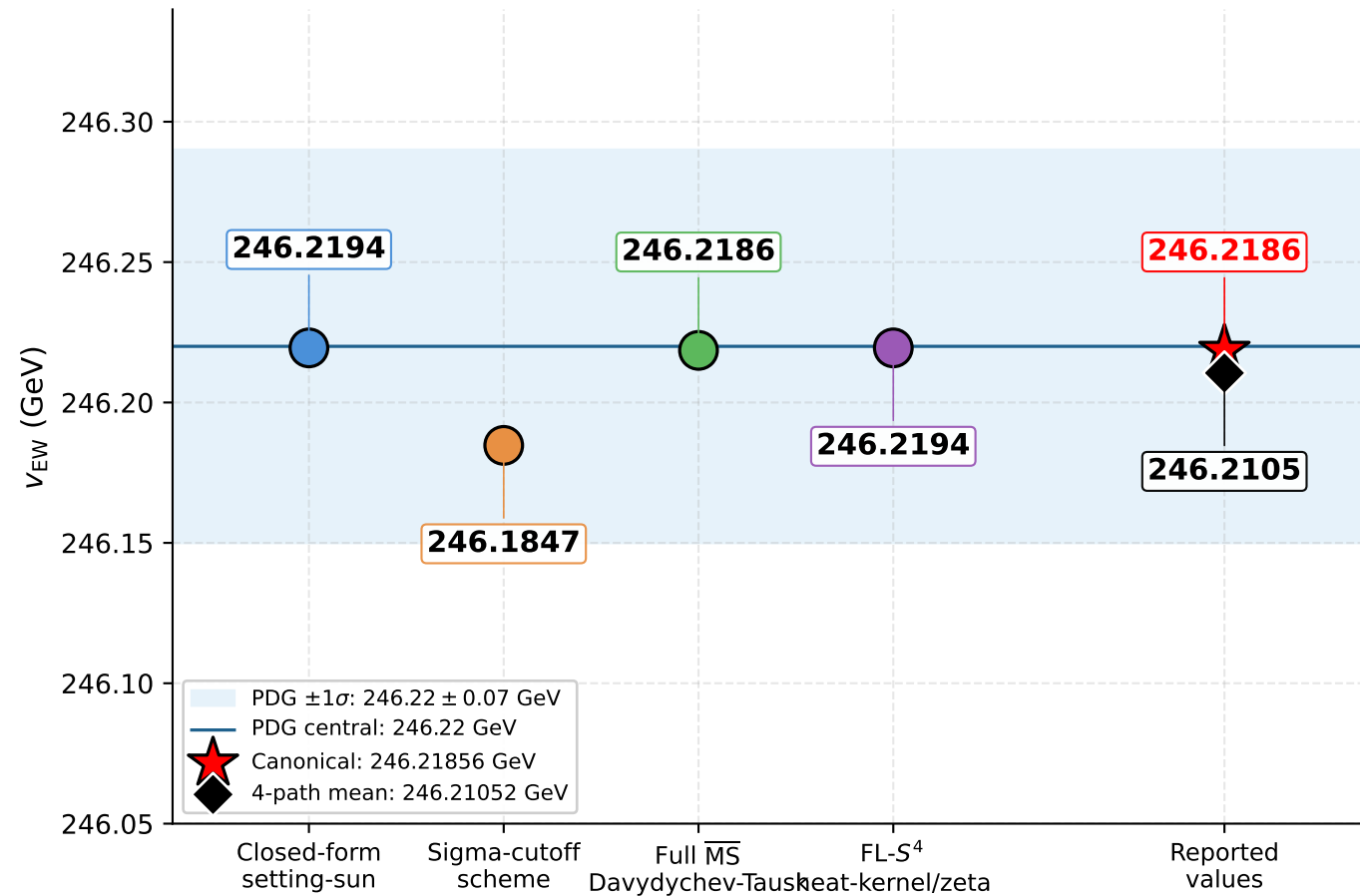
(B) Zoomed: four paths + reported values within PDG band
