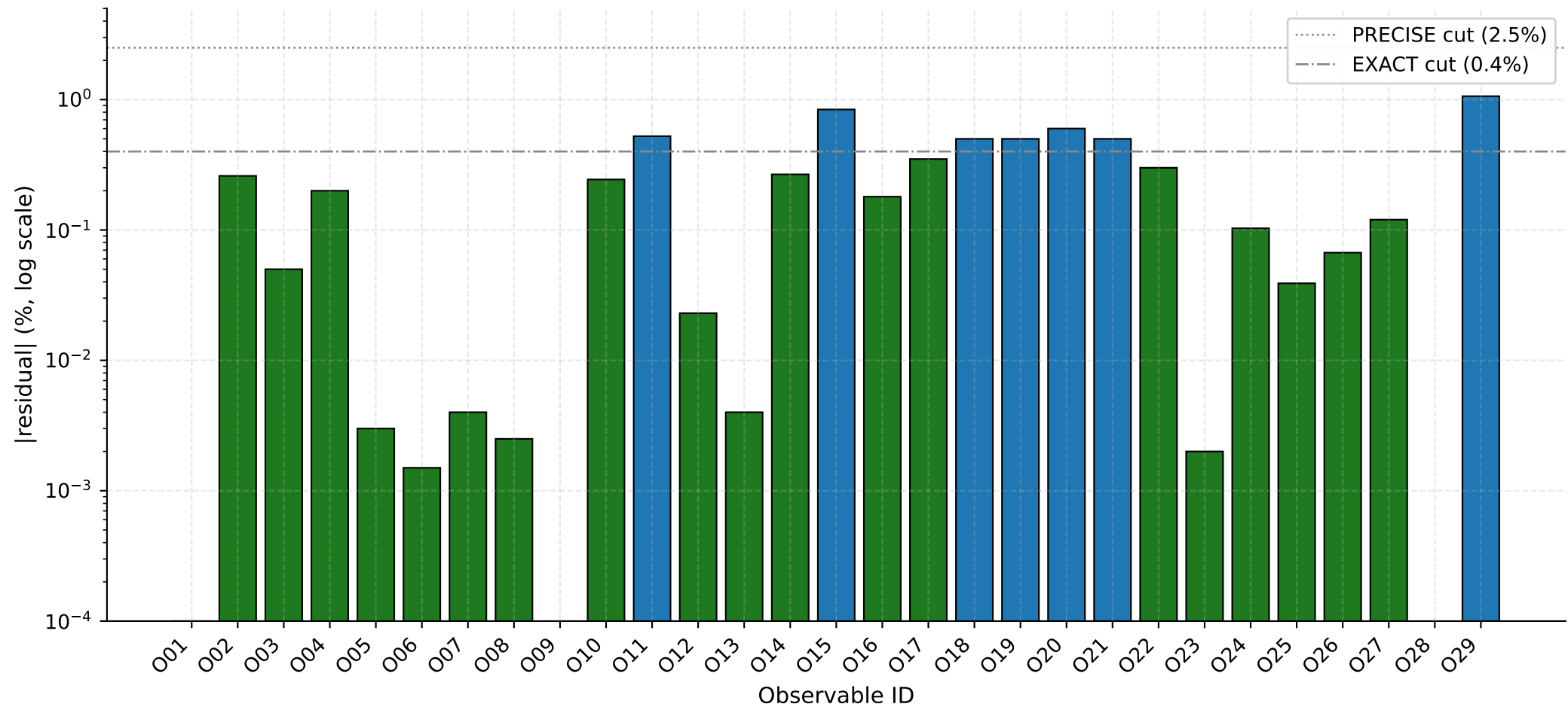
Closure-table residuals across 29 observables (22 EXACT + 7 PRECISE; 0 contradictions)
