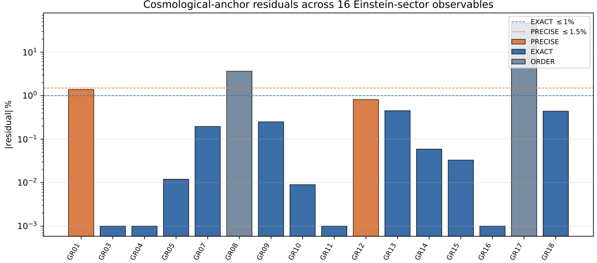
Figure 6: Anchored cosmological-anchor residuals across 16 Einstein-sector observables: 12 EXACT (residual \leq 1\% ), 2 PRECISE ( \leq 1.5\% ), 2 ORDER (binding closures); maximum EXACT/PRECISE residual 1.385% on \Omega_{\text{DM}}h^2 .
