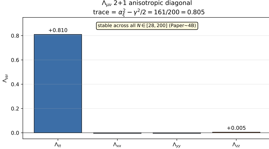
Figure 2: Cosmological-tensor diagonal \Lambda_{\mu\nu} in the 2+1 anisotropic form: time–time component \alpha_\xi^2 = 81/100 , two negative spatial axes -\gamma^2/2 = -1/200 , one positive spatial axis +\gamma^2/2 = +1/200 ; trace = \alpha_\xi^2 - \gamma^2/2 = 161/200 = 0.805 .
