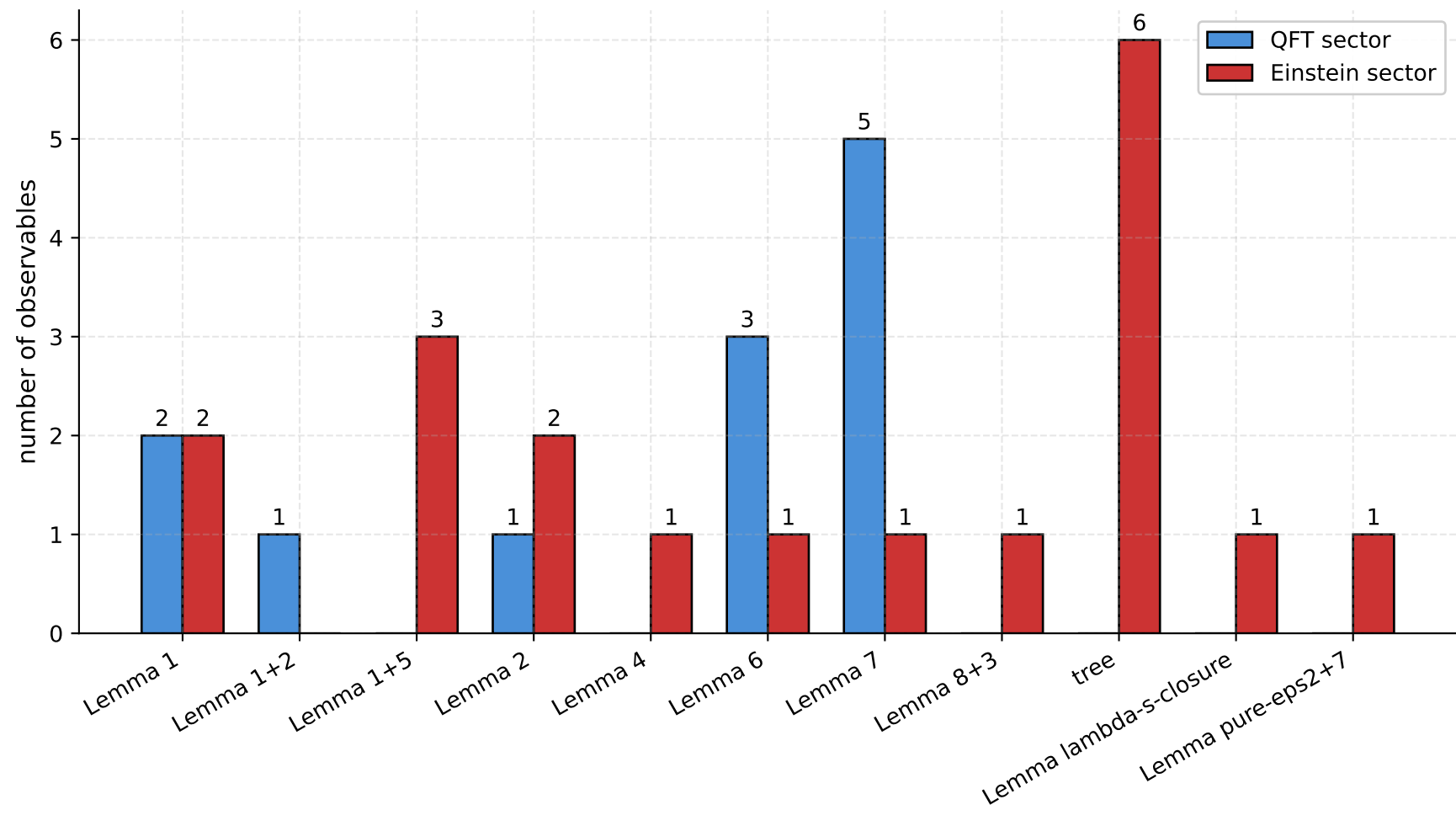
QFT sector vs Einstein sector inventory by lemma class
