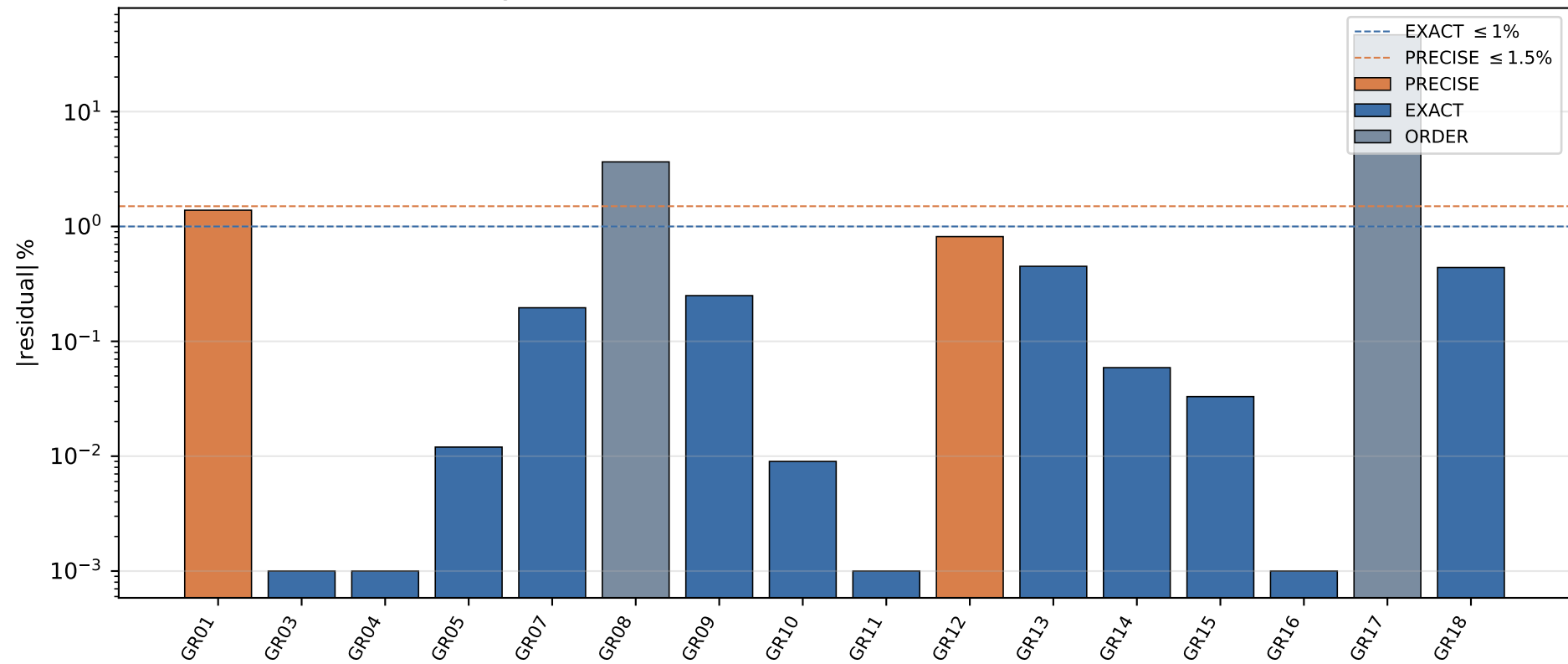
Cosmological-anchor residuals across 16 Einstein-sector observables
