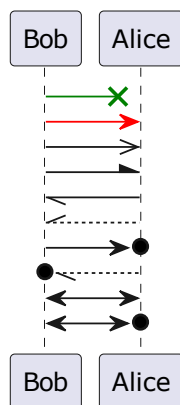
Figure 2: Types of arrows
