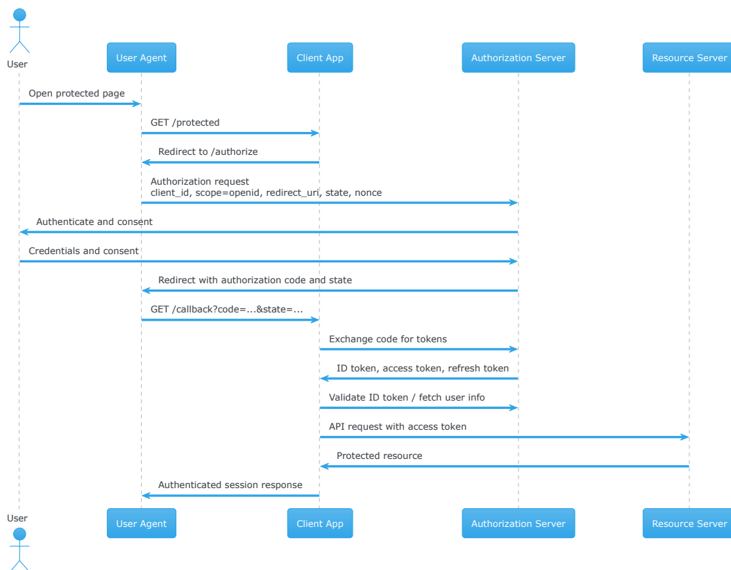
Figure 8: OIDC Authorization Code Flow
