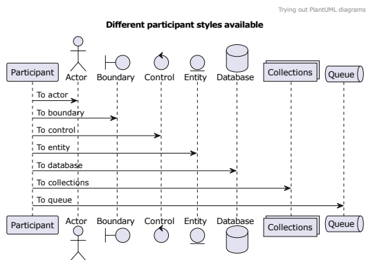
Figure 1: Types of participants supported by PlantUML
