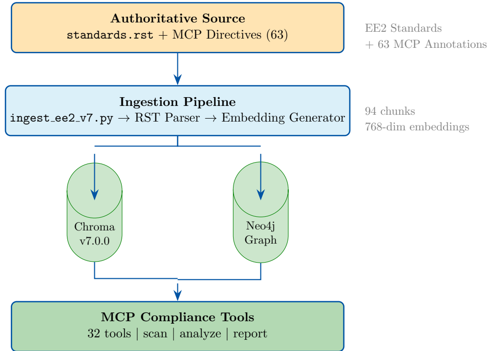
Figure 1: MCP Semantic Annotation Architecture (v7.0.0)
