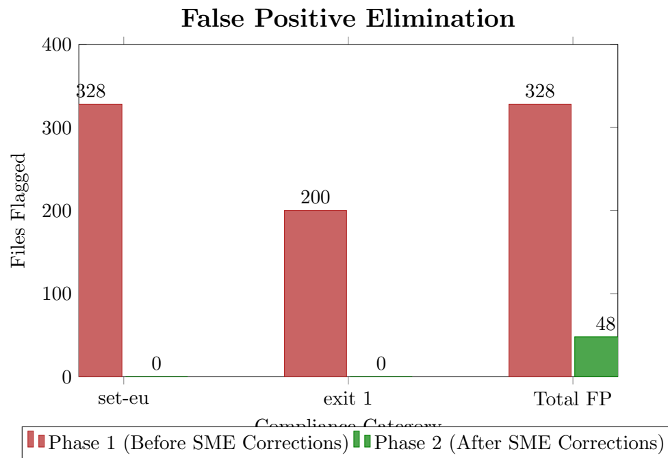
Figure 3: 85% Reduction in False Positives Through Semantic Annotations
