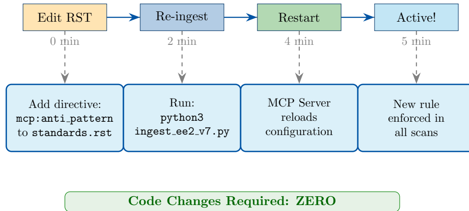
Figure 7: 5-Minute Update Workflow with Zero Code Changes
