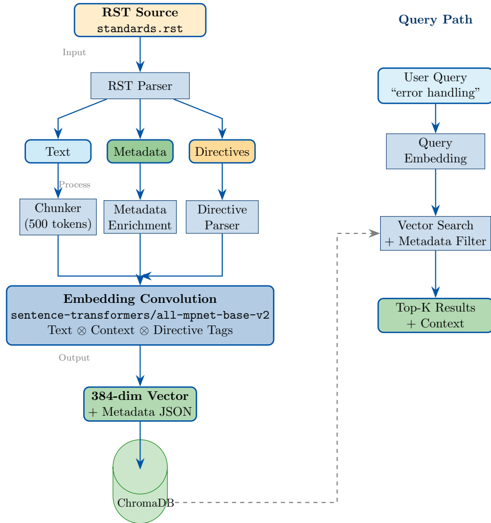
Figure 2: Embedding Convolution: How RST Directives Become Searchable Vectors
