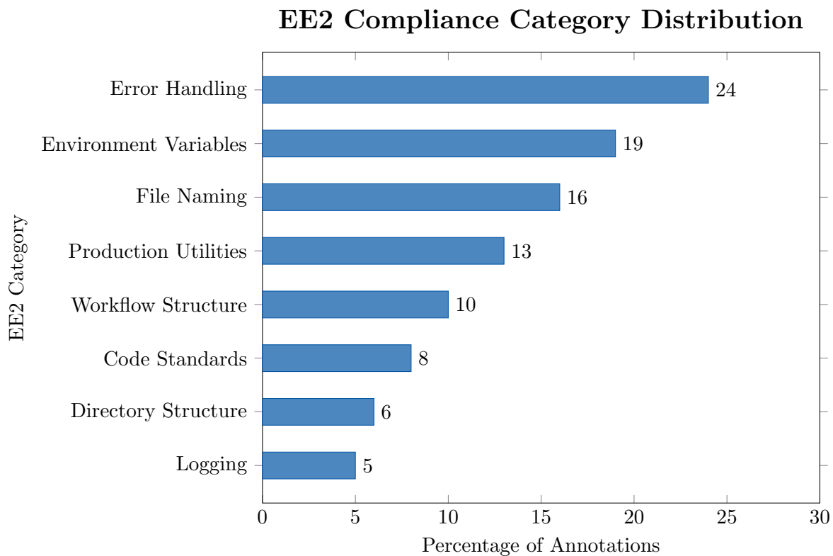
Figure 5: Distribution of Annotations Across EE2 Compliance Categories (63 total directives)
