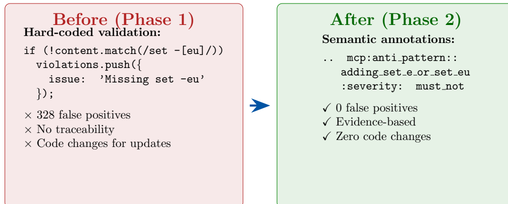
Figure 8: Transformation from Hard-Coded to Semantic Validation
