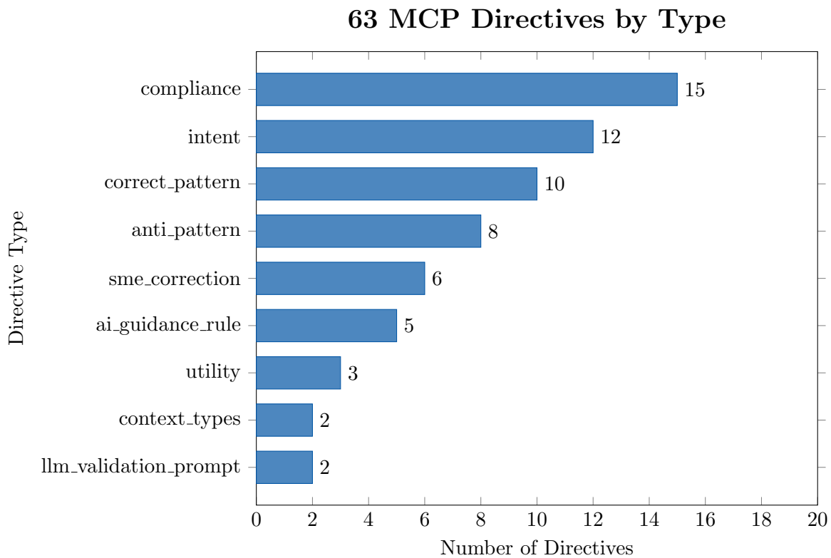
Figure 4: Distribution of MCP Directive Types in standards.rst
