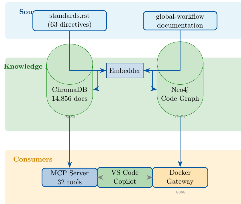
Figure 6: MCP-RAG System Components and Data Flow
