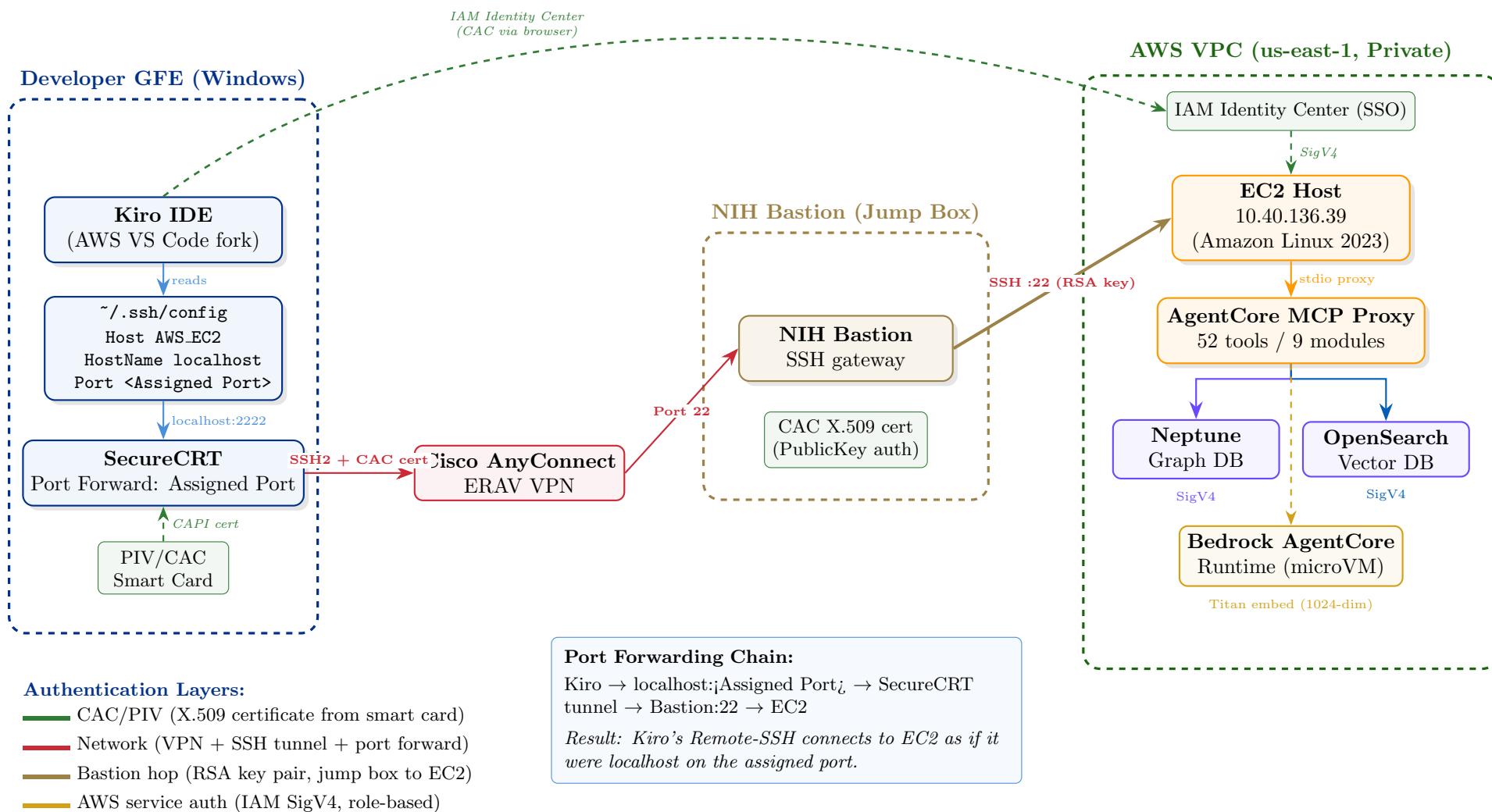
Figure 1: End-to-end connectivity: Kiro IDE on GFE laptop through CAC-authenticated bastion hop to AWS EC2 and MCP infrastructure
