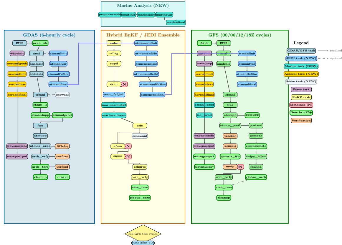
Figure 1: Global Model Parallel Sequencing v17+ — Updated from v16 with JEDI, Marine, and Aerosol Analysis Systems
