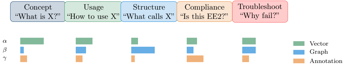
Figure 4: Query type detection adjusts retrieval weights automatically
