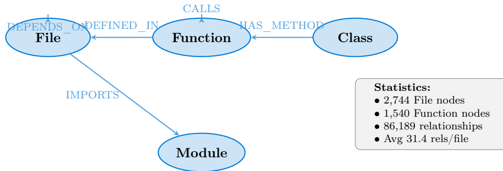
Figure 3: Neo4j graph schema showing node types and relationships
