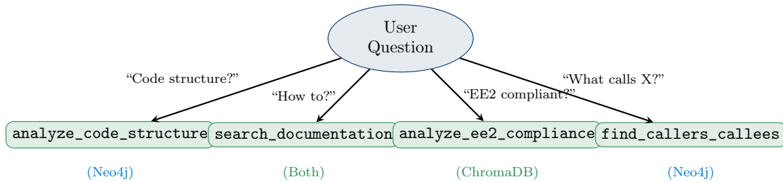
Figure 6: Tool selection based on user question type
