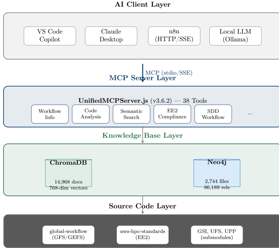
Figure 1: MCP/RAG System Architecture — Four-layer design with COTS LLM independence
