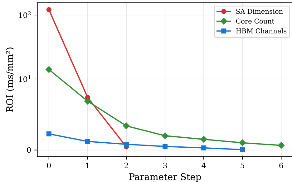
(a) Prefill Latency ROI
