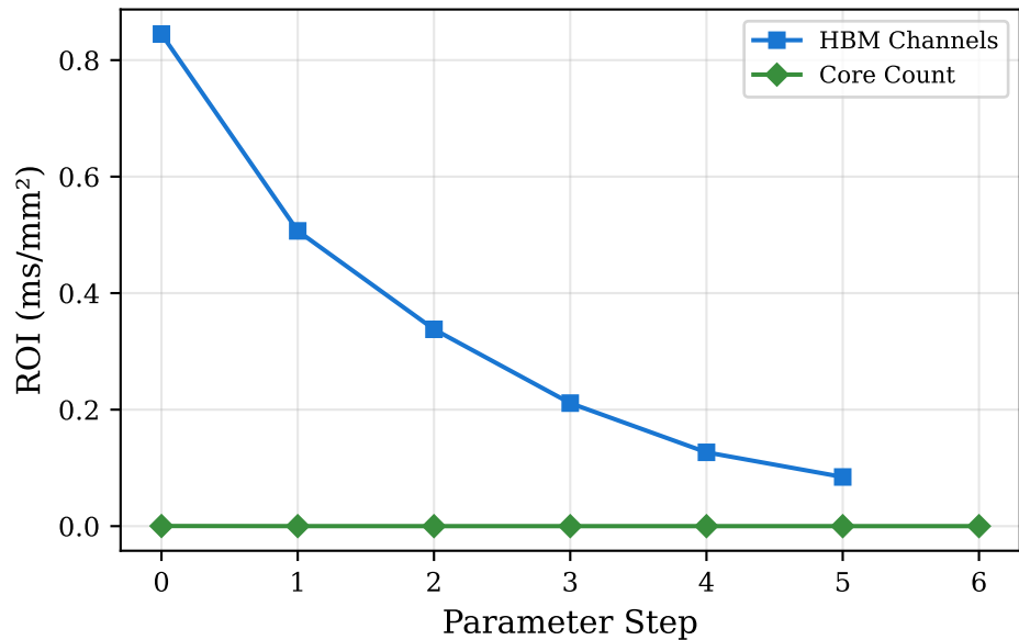
(b) Decode Latency ROI
