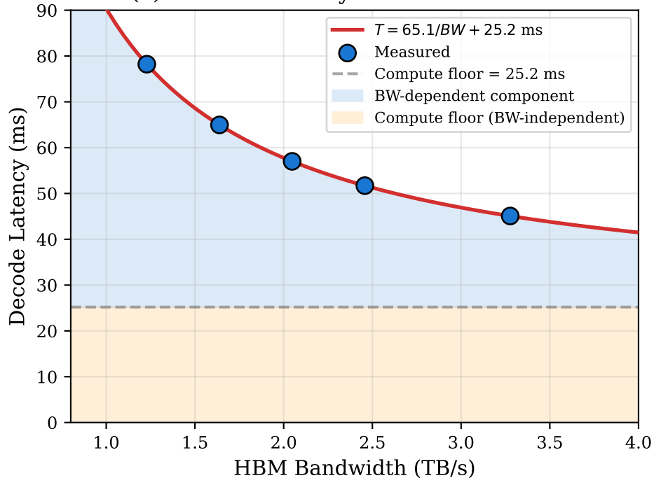
(a) Decode Latency vs HBM Bandwidth
