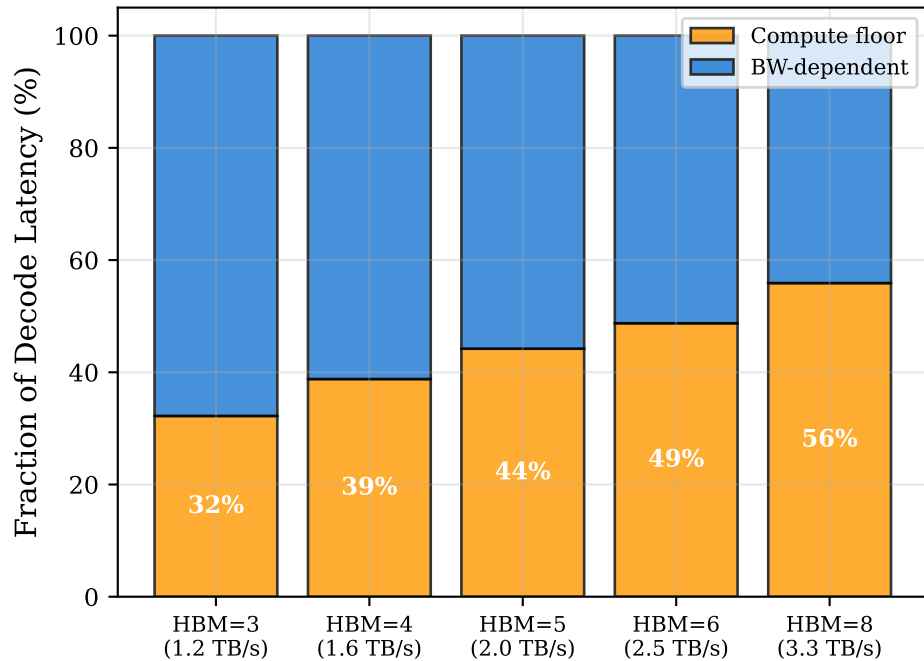
(b) Compute Floor Dominance
