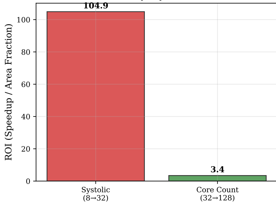
(b) Area-Efficiency: Systolic is 31x better
