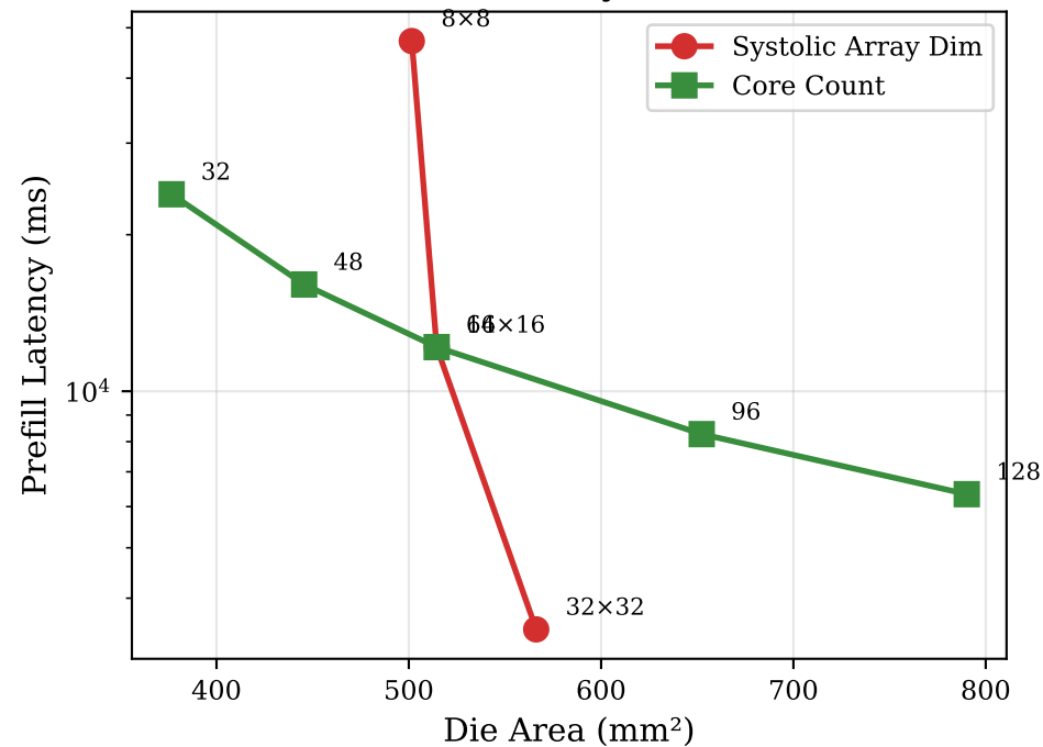
(a) Prefill Latency vs Die Area
