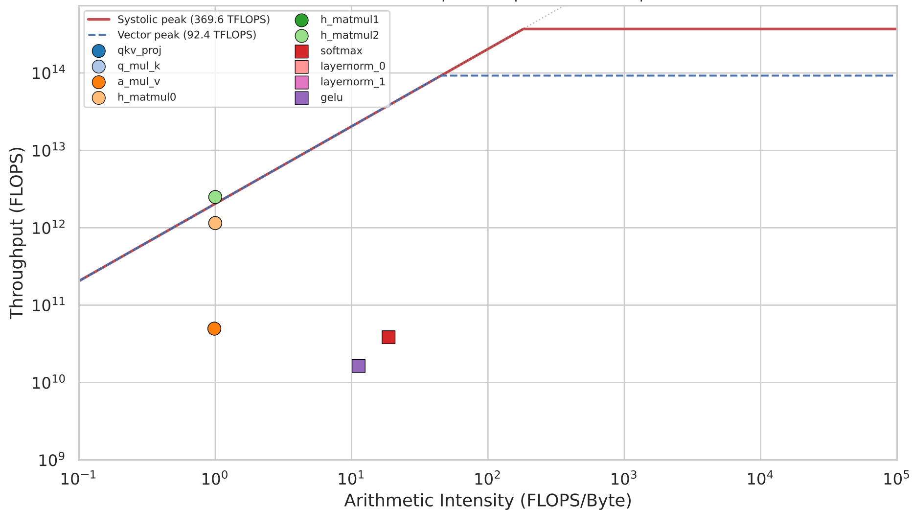
Roofline — LLaMA-7B | decode | BS=1 SL=128 | 1x GPU
