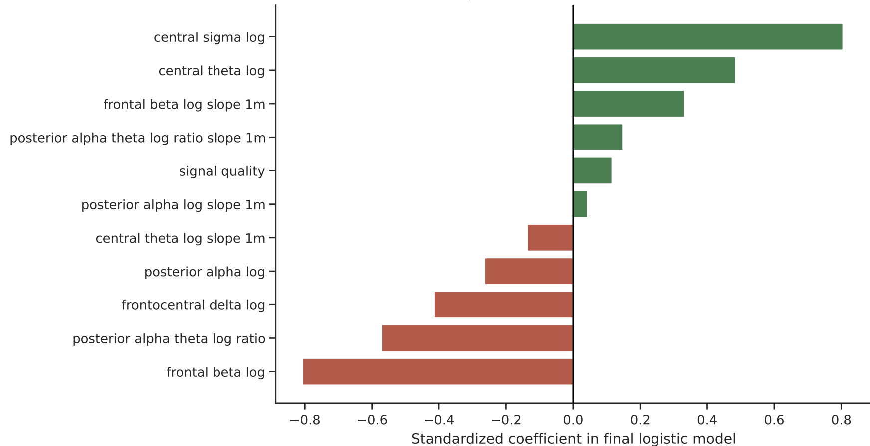
Interpretable EEG feature contributions
