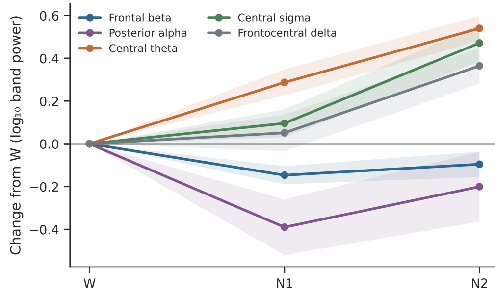
A PSD-derived physiological profiles
