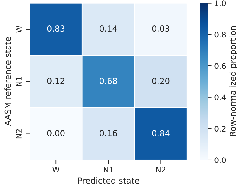
C LOSO confusion matrix: dynamic logistic model
