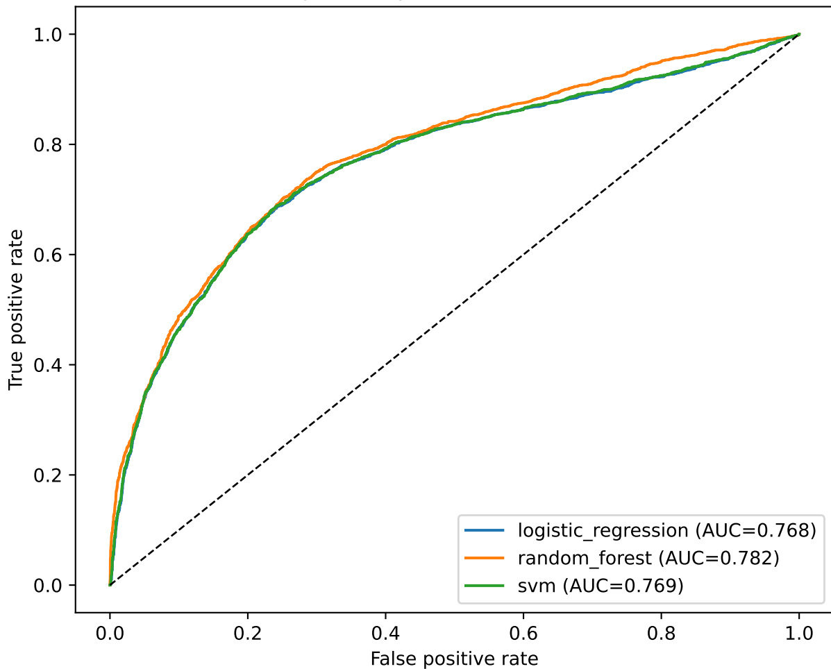
Leave-one-subject-out prediction of N2 within 5 minutes
