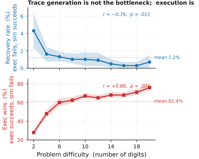
Figure 6. Recovery mass (blue) < 2% on average and reduces as tasks get harder. On the other hand, LLM execution gets noisier compared to python execution (red) . Recovery rate \Pr(\neg C) r (Code Execution Fails but LLM Reasoning succeeds | Incorrect Code) in blue trends down. Exec wins \Pr(C) e_C (Code Execution succeeds and LLM reasoning fails | Correct Code) increases as tasks get harder.
