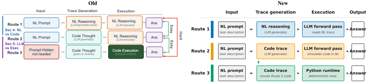
Figure 1. Three-Route Framework. We decompose algorithmic reasoning into: (1) Translation into NL or code, and (2) Execution via LLM or solver. This yields three routes: Route 1 (Direct NL), Route 2 (Code + NL simulation), Route 3 (Code + Solver Execution). Prior work compares only Route 1 vs. Route 3, confounding translation and execution. Our Route 2 isolates these factors.
