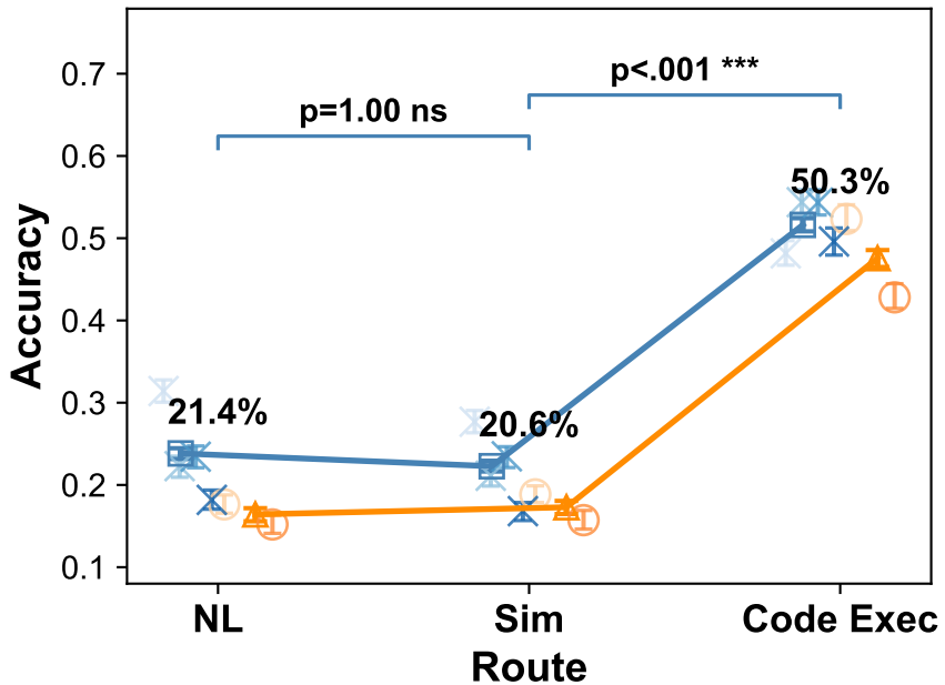
(A) Accuracy Across Routes
