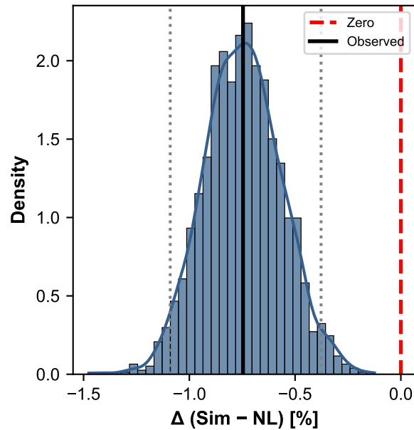
(B) \Delta = -0.75\% [-1.09, -0.38]
