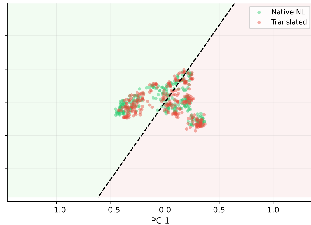
Claude Sonnet 4.5 Acc=97.0% AUC=0.998
