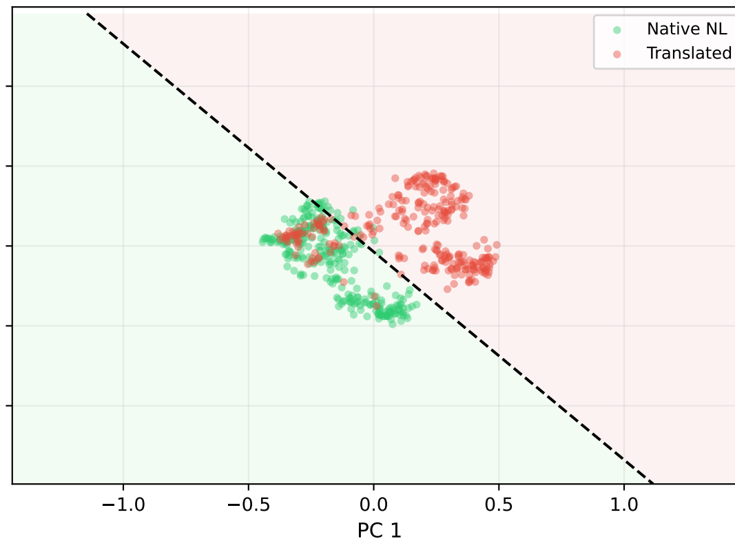
Gemini 2.0 Flash Acc=96.9% AUC=0.996
