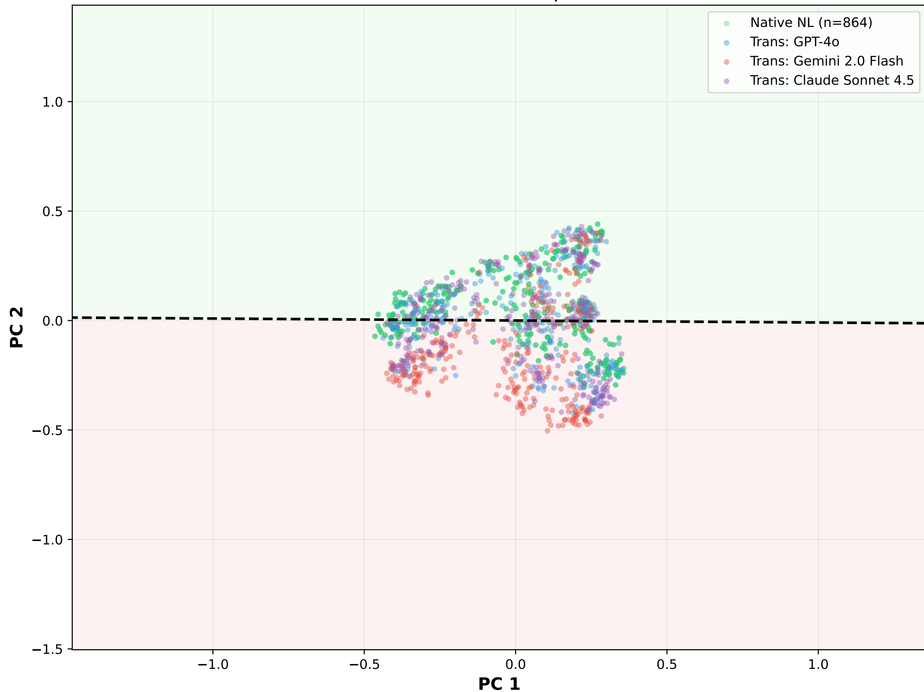
Native NL vs Translated (3 translators pooled) Full-dim: Acc=95.9% AUC=0.992 | 2-D PCA: Acc=58.0%
